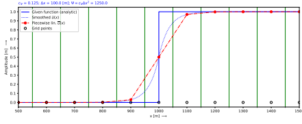
(a) Step defined at cell centre.
