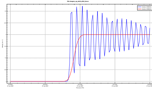
(a) Time histories of the velocity for the observation point at the centre of the domain, x = 10\,000 \text{ [m]} . The blue line, without artificial viscosity and the red line with artificial velocity.
