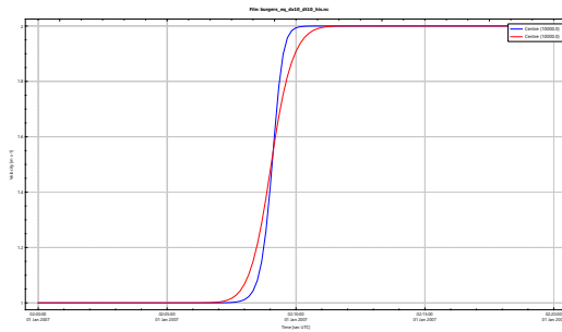
(a) Time histories of the velocity for the observation point at the centre of the domain, x = 10\,000 [m]. The blue line, without artificial viscosity and the red line with artificial velocity.
