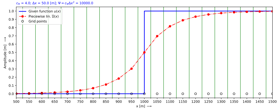
Figure 4.9: Step function approximated by a piecewise linear function (red line with dots at the nodes), c_\Psi = 4 , \Delta x = 50 [m] and \Psi = 10000 . The thin green vertical lines indicate the borders of the finite volumes.
