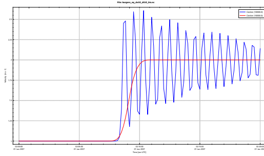
(a) Time histories of the velocity for the observation point at the centre of the domain, x = 10\,000 \text{ [m]} . The blue line, without artificial viscosity and the red line with artificial velocity.
