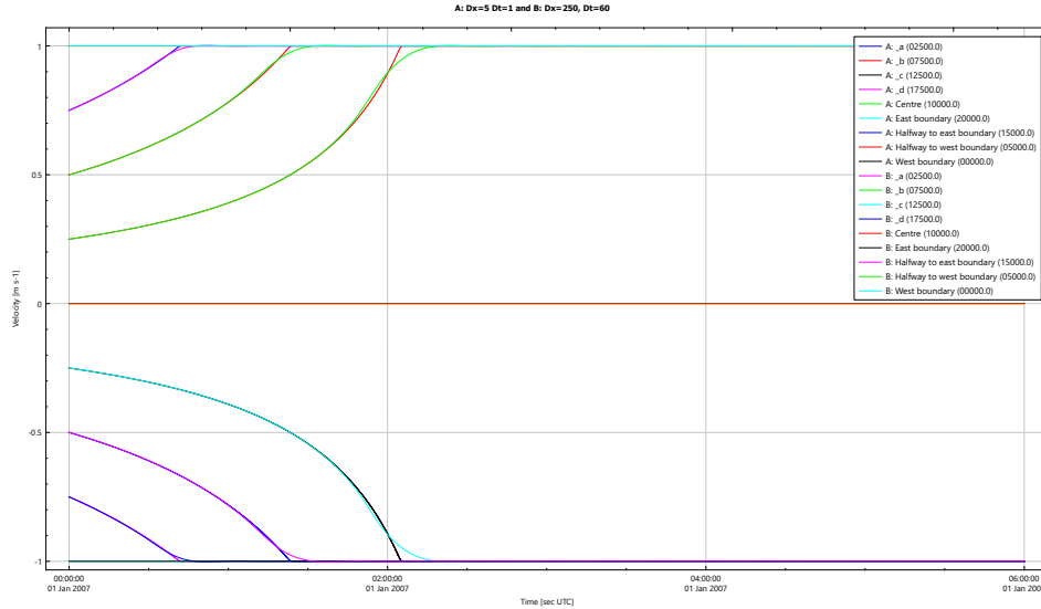
Figure 6.14: Time history for a simulation with \Delta x = 5 [m], \Delta t = 1 [s] and \Delta x = 250 [m], \Delta t = 60 [s]
