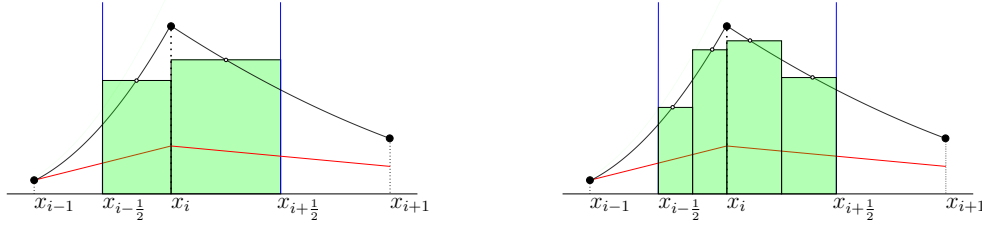
(a) Quadratic function approximated by 1-point Gauss.
