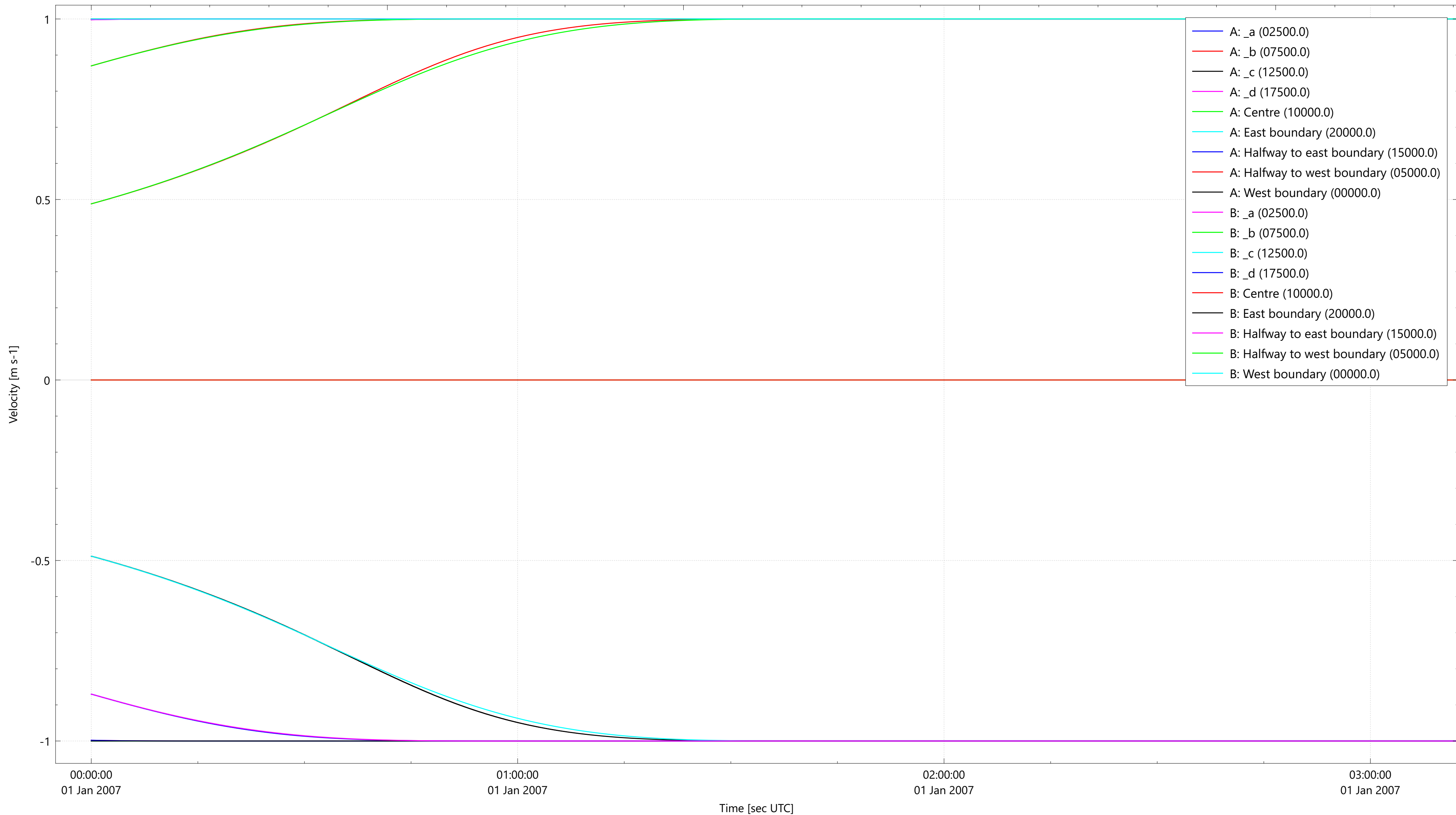
Time histories Burgers equation
