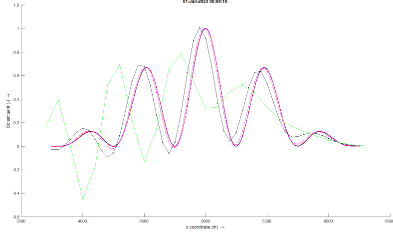
Figure 6.9: Wave package experiment, results at t = 250 [s] and \Delta t = 0.01 [s]: Blue: \Delta x = 5 [m], Red: \Delta x = 10 [m], Cyan: \Delta x = 25 [m], Black: \Delta x = 50 [m], Green: \Delta x = 100 [m].
