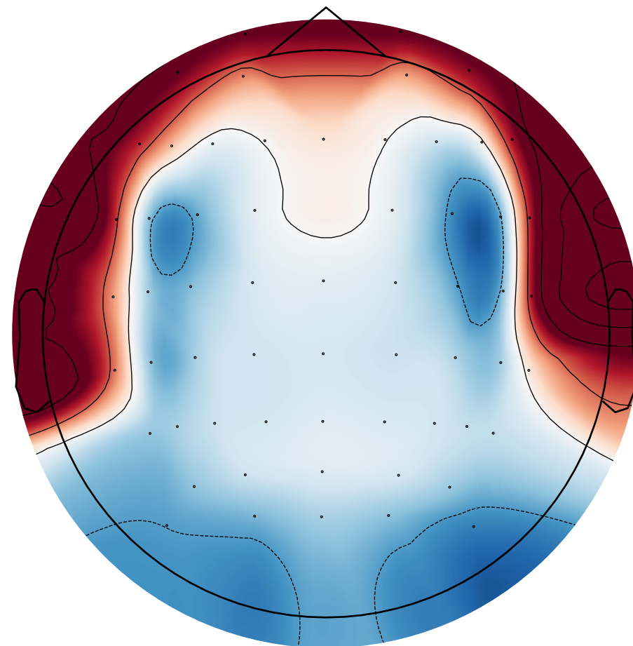
Beta (13-30 Hz) Mean Waveform Asymmetry (N=215)
