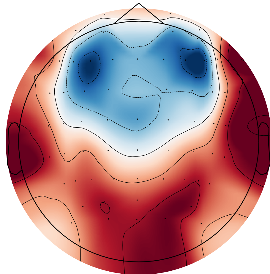
Alpha (8-13 Hz) Mean Waveform Asymmetry (N=215)
