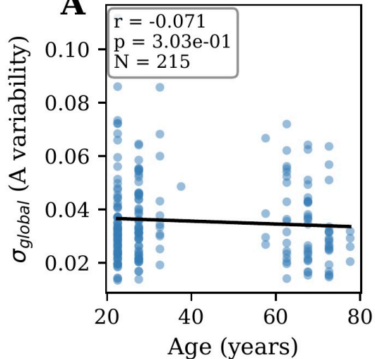
Global variability ~ age
