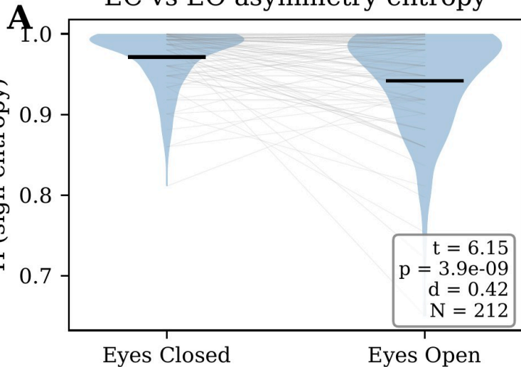
EC vs EO asymmetry entropy
