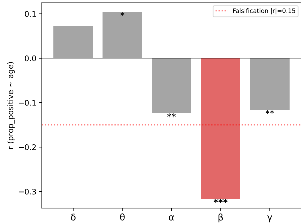
B. Band Specificity: \beta strongest (CONFIRMED)
