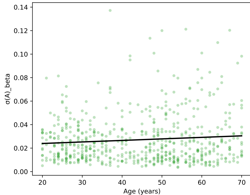
C. Variability: r = +0.091 , p = 0.026 Predicted: r > 0 — CONFIRMED
