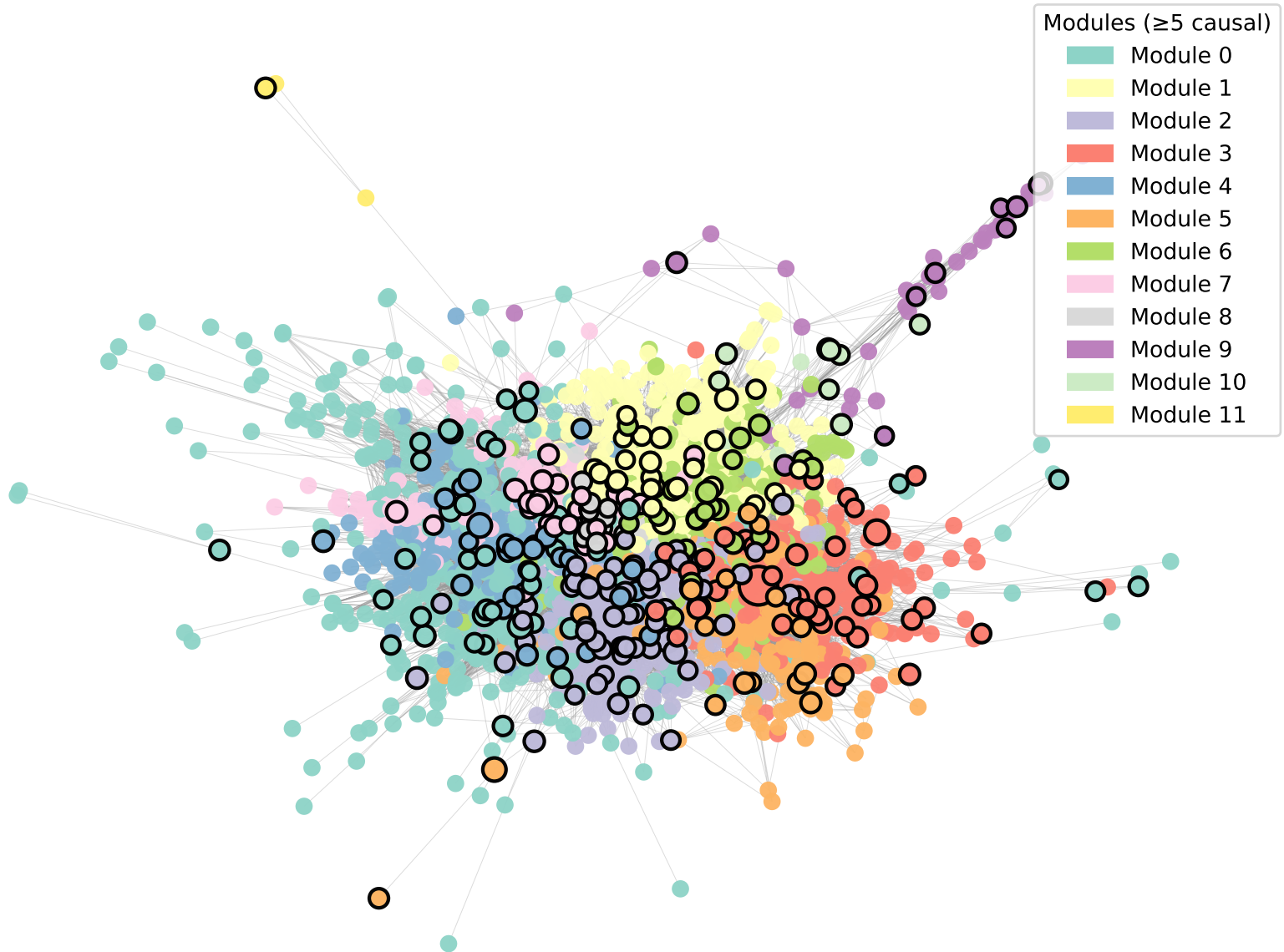
Largest causal subnetwork — modules with \geq 5 causal gene
