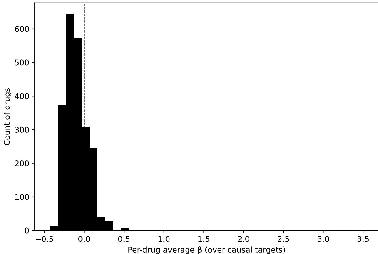
Histogram of per-drug avg \beta — Inhibitor
