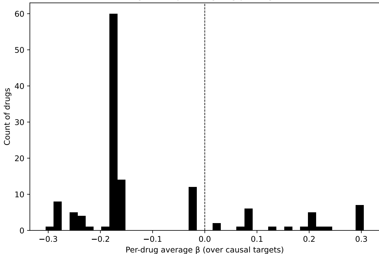
Histogram of per-drug avg \beta — Agonist
