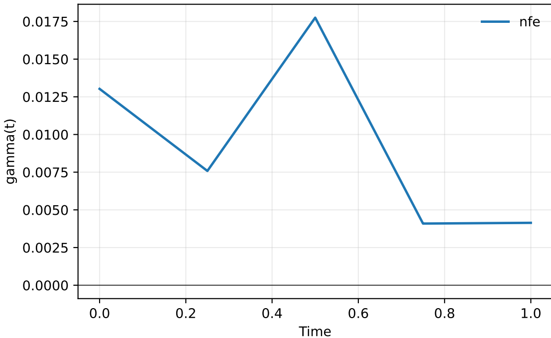
Selection trajectory
