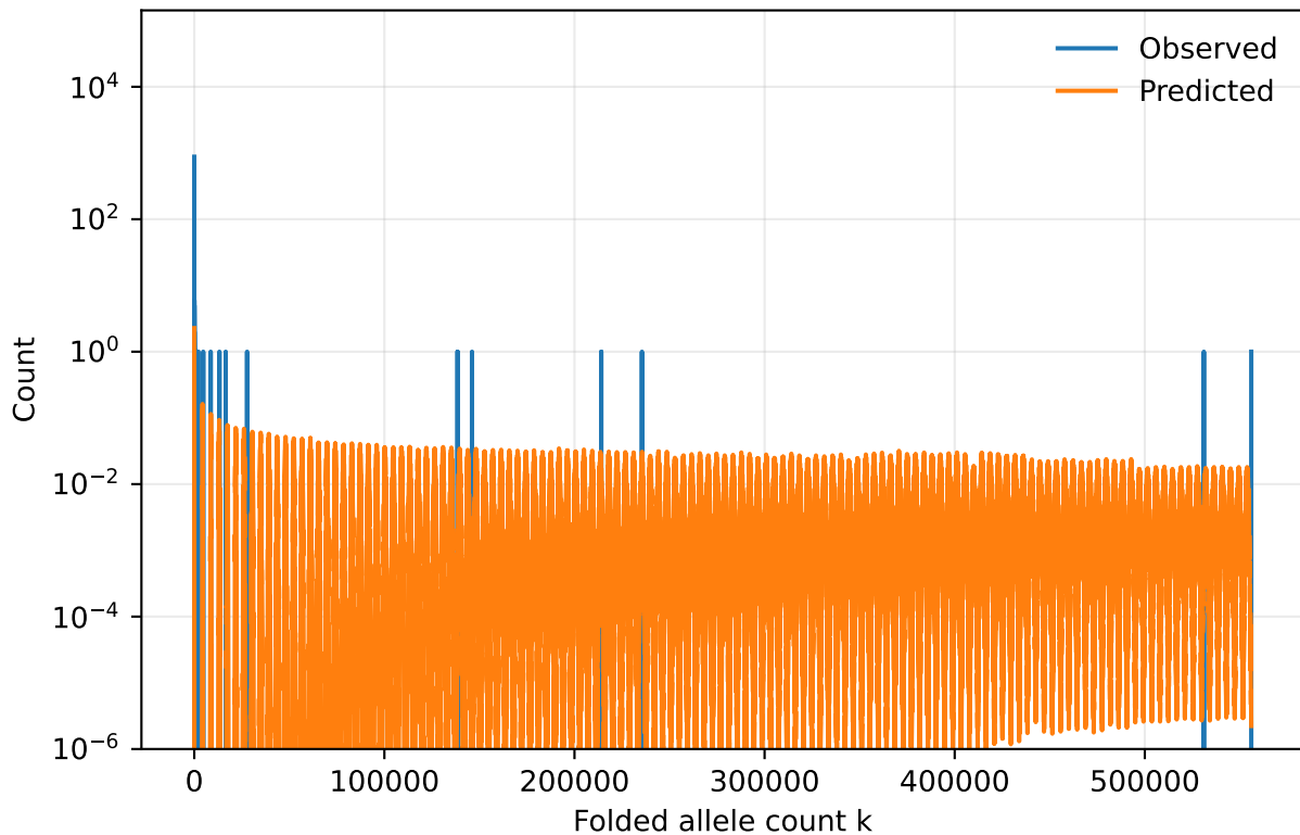
Folded SFS nfe
