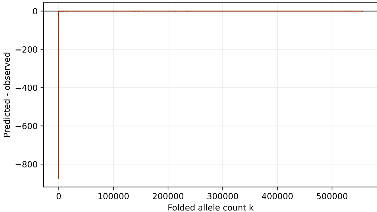
Folded SFS residuals
