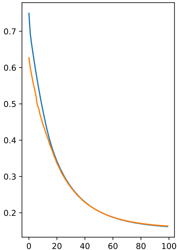
Reconstruct Loss for ATAC Pretrain
