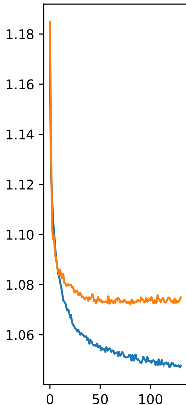
Reconstruct Loss for Train KL Divergence for TrainDiscriminator Loss for Train
