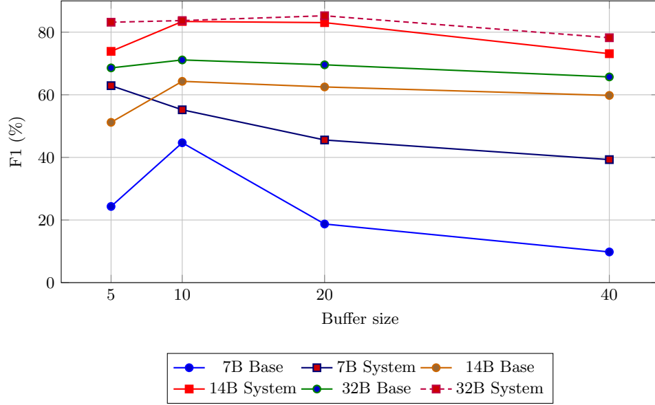
Fig. 7 Context-isolation F1 across model sizes and buffer sizes. Subchat Trees improves F1 over the linear baseline in every configuration.
