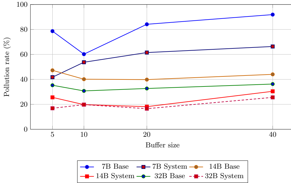
Fig. 8 Pollution rate across buffer sizes. Lower values are better. Subchat Trees consistently reduces cross-topic contamination by routing turns into branch-local buffers instead of keeping all topics in one linear transcript.
