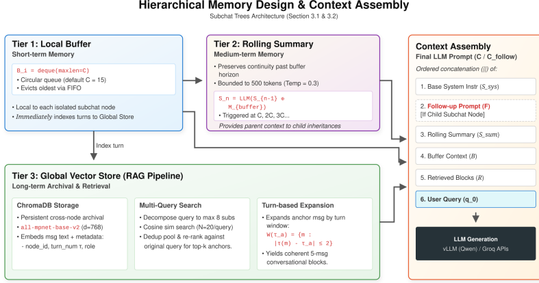
Fig. 3 Three-tier memory design showing the relationship between the LocalBuffer (circular deque), rolling summarization, and vector store archival.
