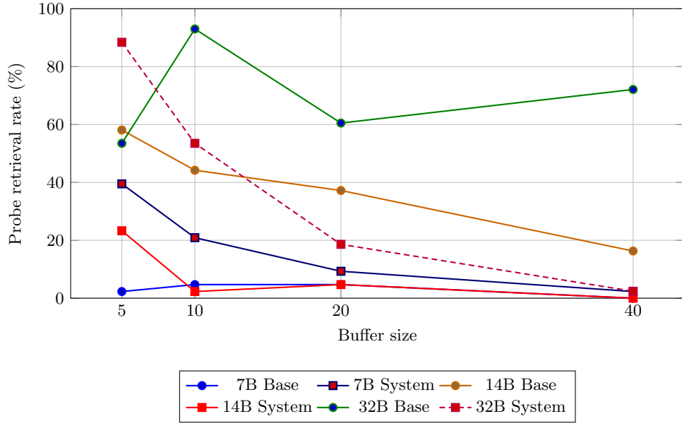
Fig. 10 RAG retrieval rate during the 43 recall probes. Probe retrieval is used as a memory-sufficiency signal because every probe asks the model to recover earlier topic content.
