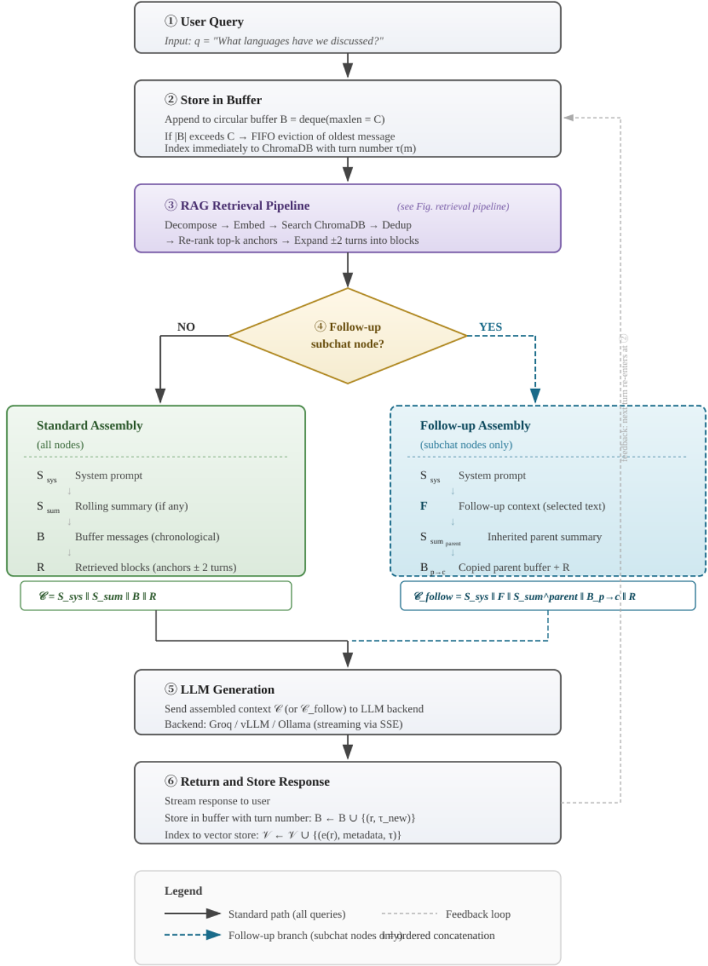
Figure 3.5: Context assembly pipeline. The user query is buffered (①–②) and passed through the RAG retrieval pipeline (③; detailed in Figure 3.4), which returns coherent context blocks R . At step ④ the pipeline branches: root-level nodes follow the standard path (solid arrows, Eq. 3.9), while follow-up subchat nodes additionally inject the selected-text prompt F and the inherited parent summary S_{\text{sum}}^{\text{parent}} (dashed arrows, Eq. 3.10). Both paths converge at step ⑤ for LLM generation, after which the response is stored back in the buffer and vector store (⑥).
