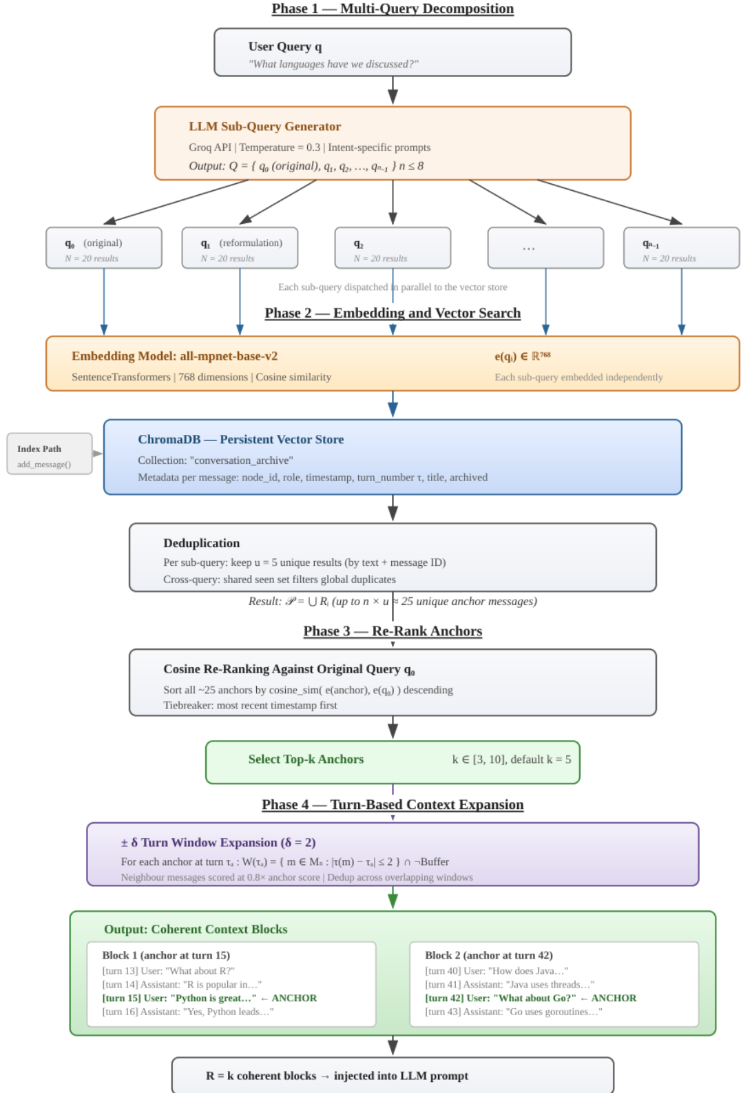
Figure 3.4: End-to-end retrieval pipeline. Phase 1: LLM-based sub-query generation decomposes the user query into up to n \leq 8 sub-queries. Phase 2: each sub-query is embedded via all-mpnet-base-v2 ( d=768 ) and dispatched to ChromaDB for cosine search ( N=20 candidates each), then deduplicated to u=5 unique results per sub-query. Phase 3: all anchor candidates are re-ranked by cosine similarity to the original query q_0 ; top- k are selected. Phase 4: each winning anchor expands \pm \delta turns ( \delta=2 ) into a coherent conversational block (Eq. 3.7). The resulting k blocks are injected into the LLM prompt.
