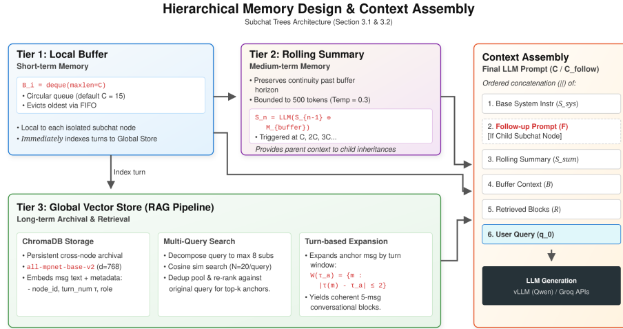
Figure 3.3: Three-tier memory design showing the relationship between the Local-Buffer (circular deque), rolling summarization, and vector store archival.
