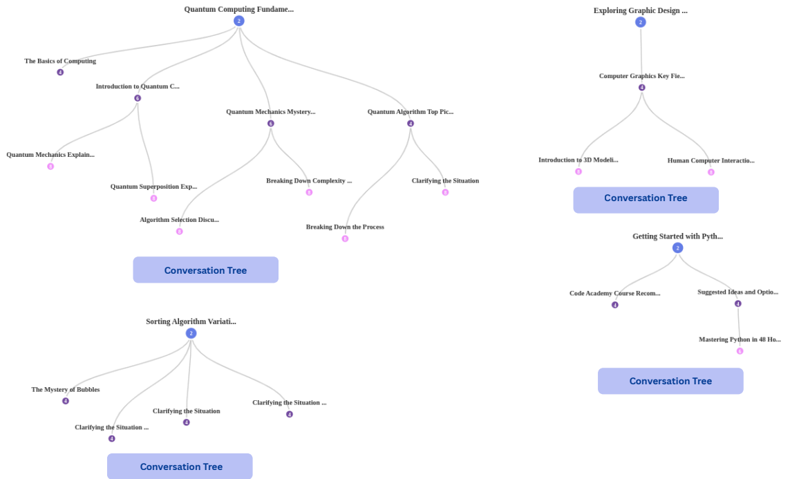
Figure 3.2: Tree view of a Conversation Forest showing multiple conversation branches. Each node represents a subchat with isolated context.
