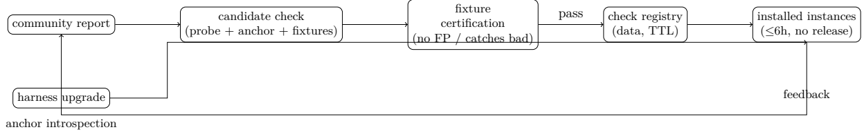
Figure 2: The check lifecycle: report \rightarrow candidate \rightarrow certify \rightarrow distribute \rightarrow verify (property 4), with introspection (property 2) guarding every upgrade.
