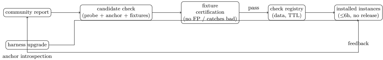
Figure 2: The check lifecycle: report \rightarrow candidate \rightarrow certify \rightarrow distribute \rightarrow verify (property 4), with introspection (property 2) guarding every upgrade.
