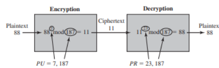
Figure 9.6 Example of RSA Algorithm
