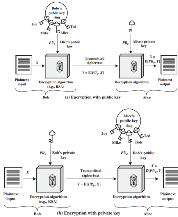
Figure 9.1 Public-Key Cryptography
