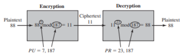
Figure 9.6 Example of RSA Algorithm
