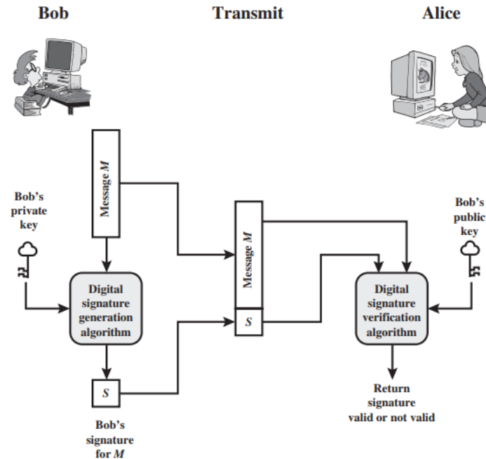
Figure 13.1 Generic Model of Digital Signature Process
