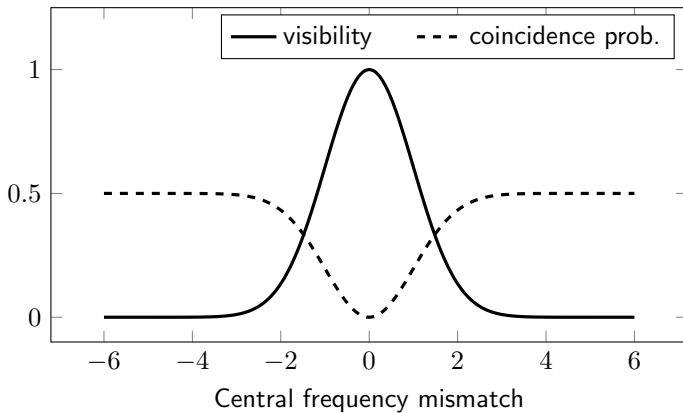
HOM interference for Case A
