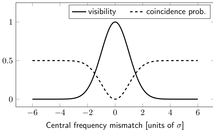
HOM interference for Case A
