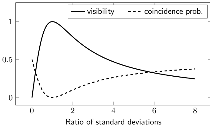
HOM interference for Case B
