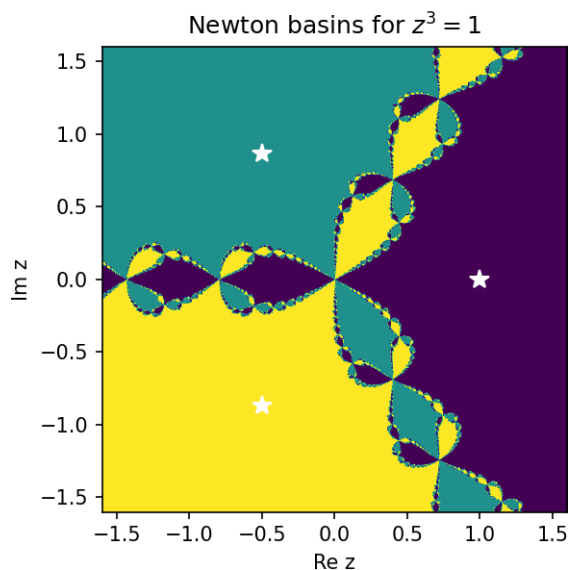
Figure 4.2: Basins of attraction of Newton's method for z^3 = 1 . Each colour shows the starting points that converge to one of the three cube roots of unity (stars). The boundaries are fractals. Produced by code/ch04/newton_fractal.py.
