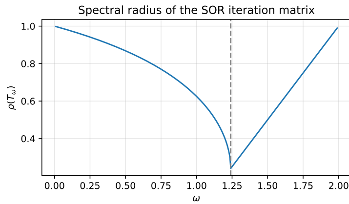
Figure 7.1: \rho(T_\omega) for Example 7.2. The minimum is sharp, at \omega_{\text{opt}} \approx 1.24 ; to the right of it \rho(T_\omega) = \omega - 1 .
