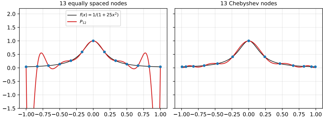
Figure 9.2: Interpolating Runge's function with 13 nodes.
