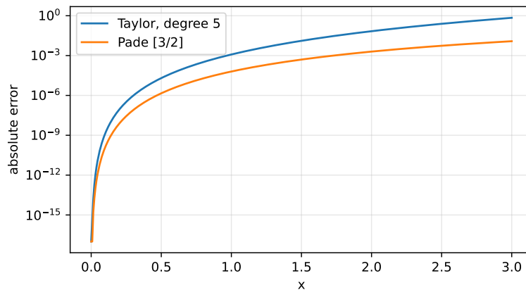
Figure 11.1: Errors of the Taylor polynomial of degree 5 and of the Padé approximant r_{3,2} for e^{-x} on [0, 3] .
