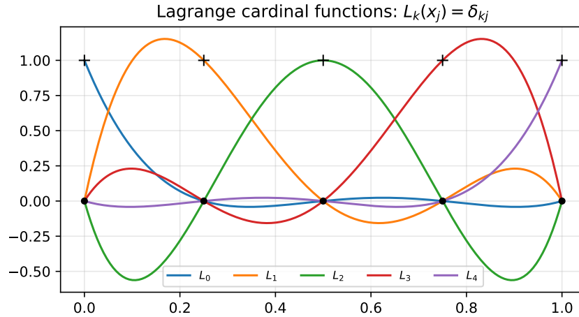
Figure 9.1: The five Lagrange cardinal functions for equally spaced nodes on [0, 1] .
