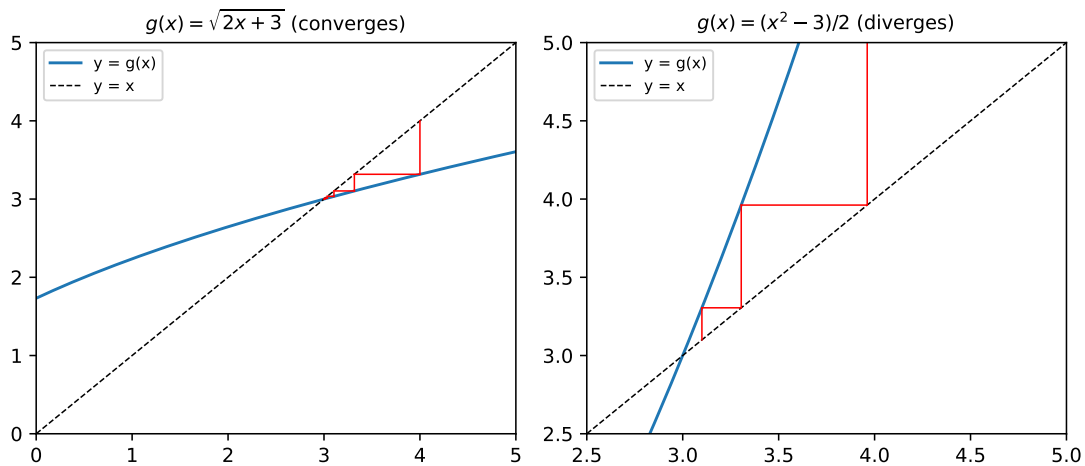
Figure 4.1: Cobweb diagrams: move vertically to the curve y = g(x) , then horizontally to the line y = x . Left: |g'| < 1 near the fixed point (convergence). Right: |g'| > 1 (divergence).
