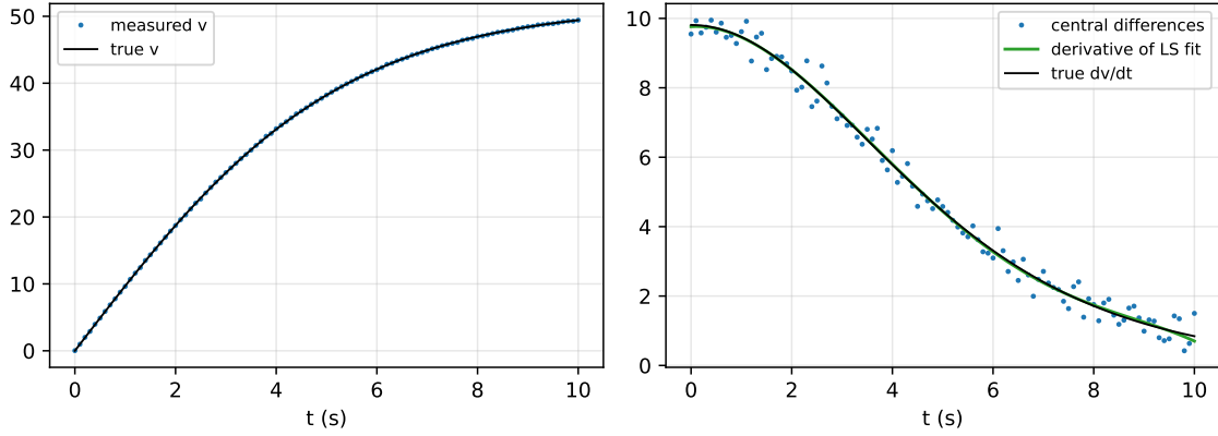
Figure 12.2: A noise level of 5 cm/s, invisible in the velocity data (left), dominates the finite-difference acceleration (right).
