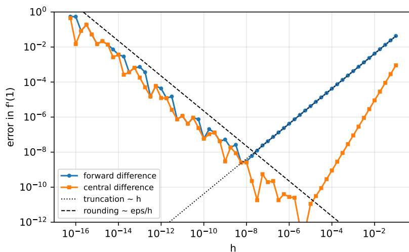
Figure 12.1: The “V-shaped” error curve of numerical differentiation for f = \sin at x = 1 . To the right of the minimum the truncation error dominates (slopes 1 and 2); to the left, rounding error dominates (slope -1 ).
