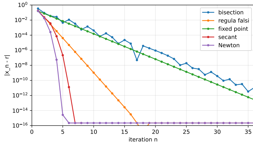
Figure 4.3: Error against iteration number on a logarithmic scale. Linear convergence appears as a straight line; superlinear convergence curves downwards.
