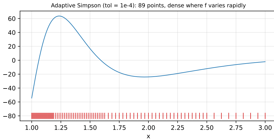
Figure 13.2: The points chosen by adaptive Simpson quadrature cluster where the integrand oscillates.
