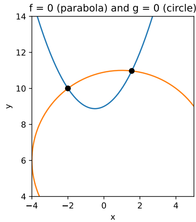
Figure 5.1: The solutions of Example 5.5 are the intersections of a parabola and a circle.
