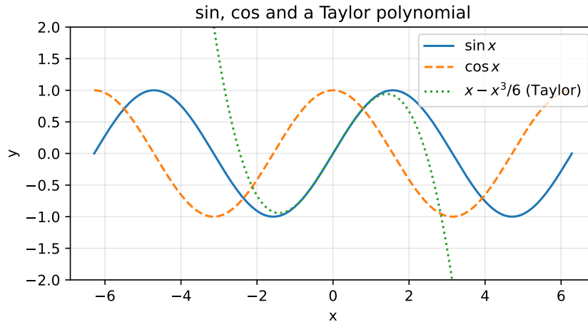
Figure 1.1: Output of Listing 1.6. The Taylor polynomial x - x^3/6 is an excellent approximation of \sin x near 0 but useless far away from 0.
