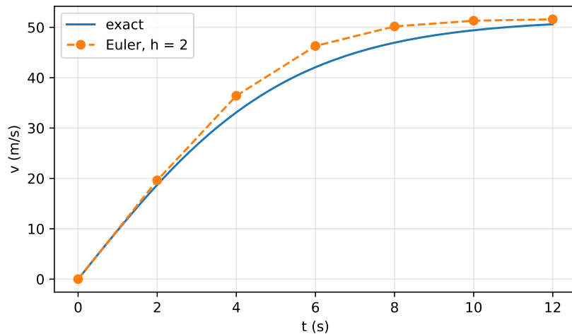
Figure 1.2: Velocity of the bungee jumper ( m = 68.1 kg, c_d = 0.25 kg/m).
