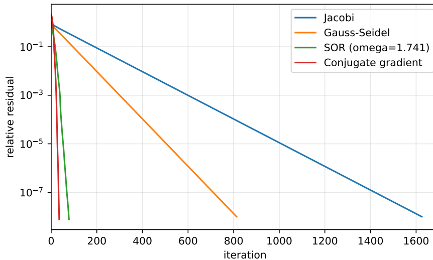
Figure 7.3: Convergence histories for the Poisson problem with m = 20 .
