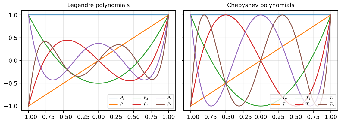
Figure 10.3: The first six Legendre and Chebyshev polynomials.
