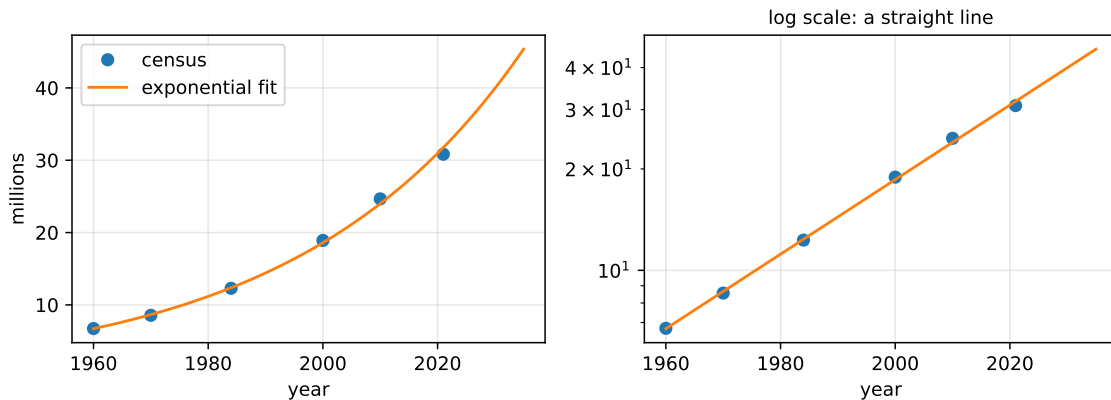
Figure 10.2: Exponential growth model for the population of Ghana.
