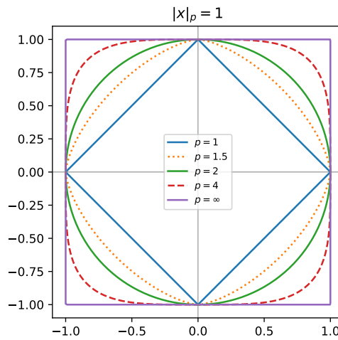
Figure 8.1: Unit circles \{\mathbf{x} \in \mathbb{R}^2 : \|\mathbf{x}\|_p = 1\} . As p increases they grow from the diamond ( p = 1 ) to the square ( p = \infty ).
