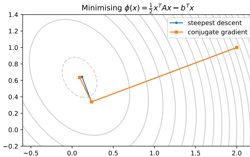
Figure 7.2: Steepest descent zig-zags towards the minimum; conjugate gradients reaches it in n = 2 steps.
