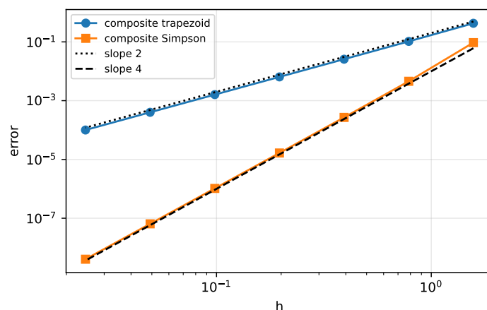
Figure 13.1: Errors of the composite rules for \int_0^\pi \sin x \, dx : slopes 2 and 4 on a log-log plot.
