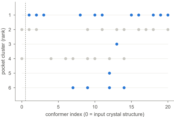
a detection is per conformer; clusters span the ensemble
