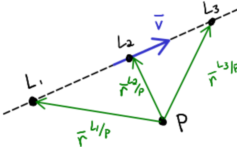
Fig. 14.2: \bar{v} is bound to a line L . The moment can be calculated based on a position vector from P to any point on the line, for example L_1 , L_2 or L_3 as shown.
