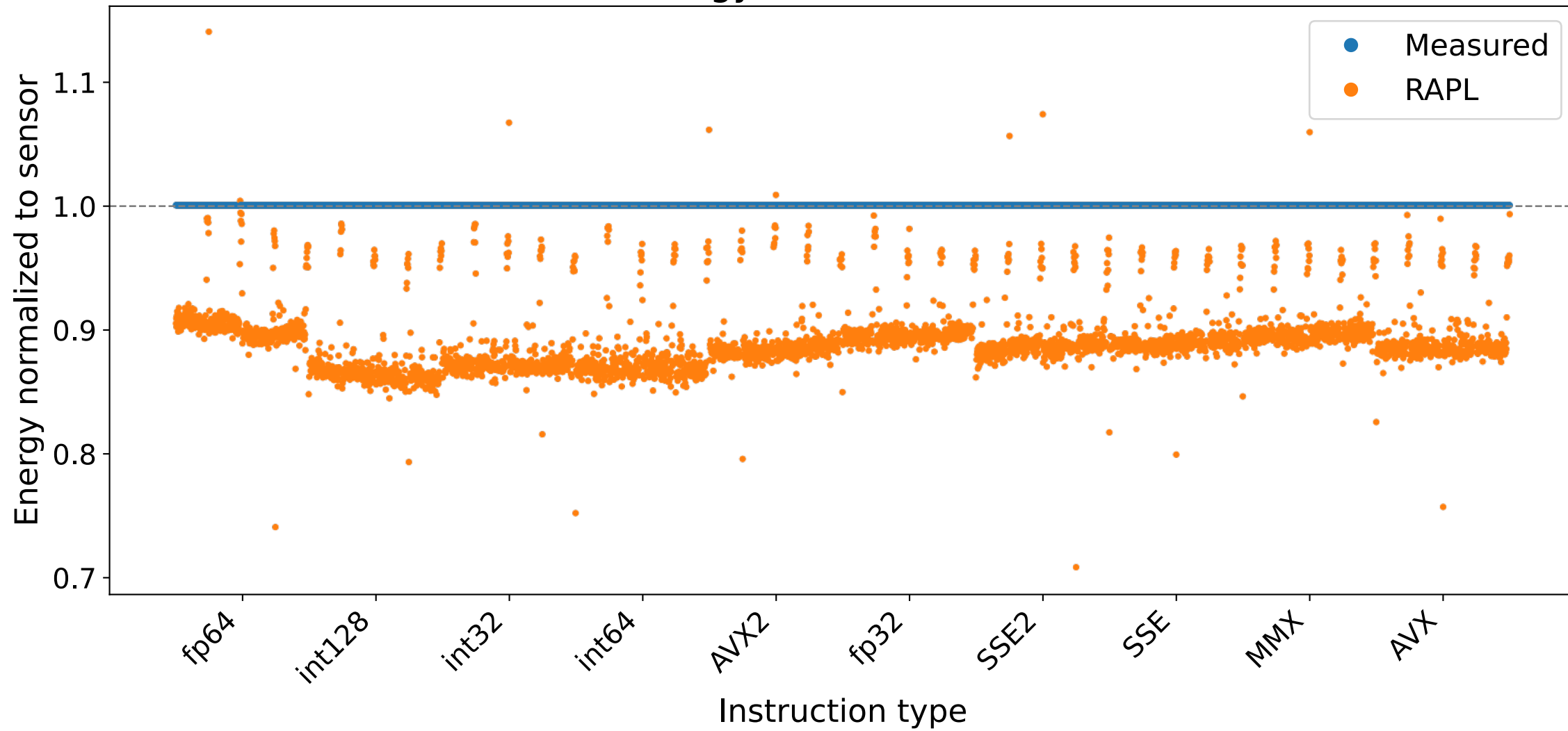
RAPL vs measured energy, normalized to sensor (Arrow Lake)
