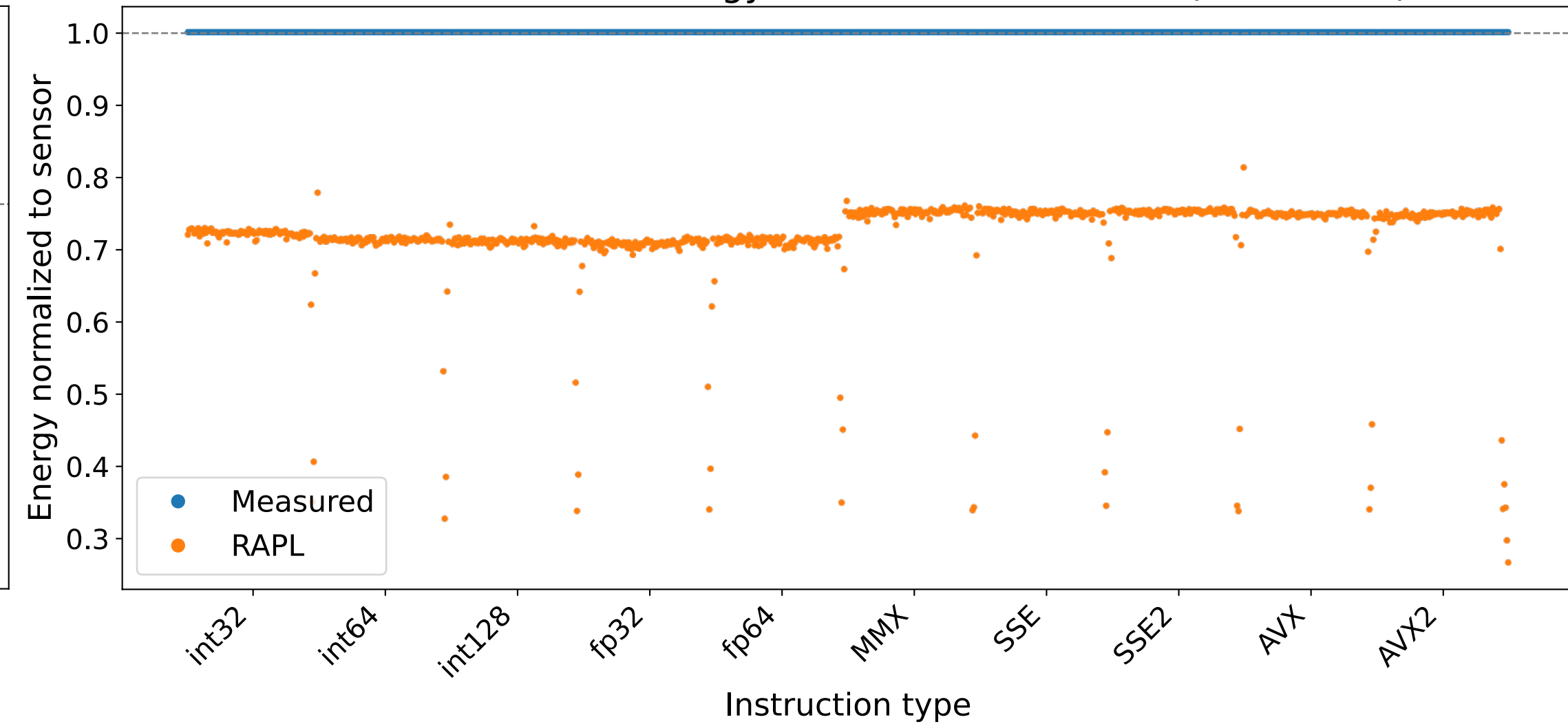
RAPL vs measured energy, normalized to sensor (Coffeelake)
