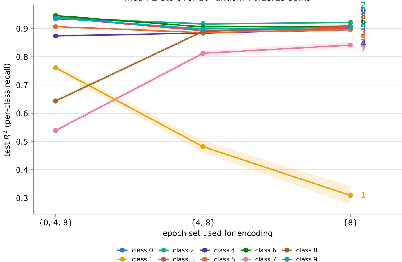
Per-class recall prediction from SANE embeddings mean \pm std over 10 random 70/15/15 splits
