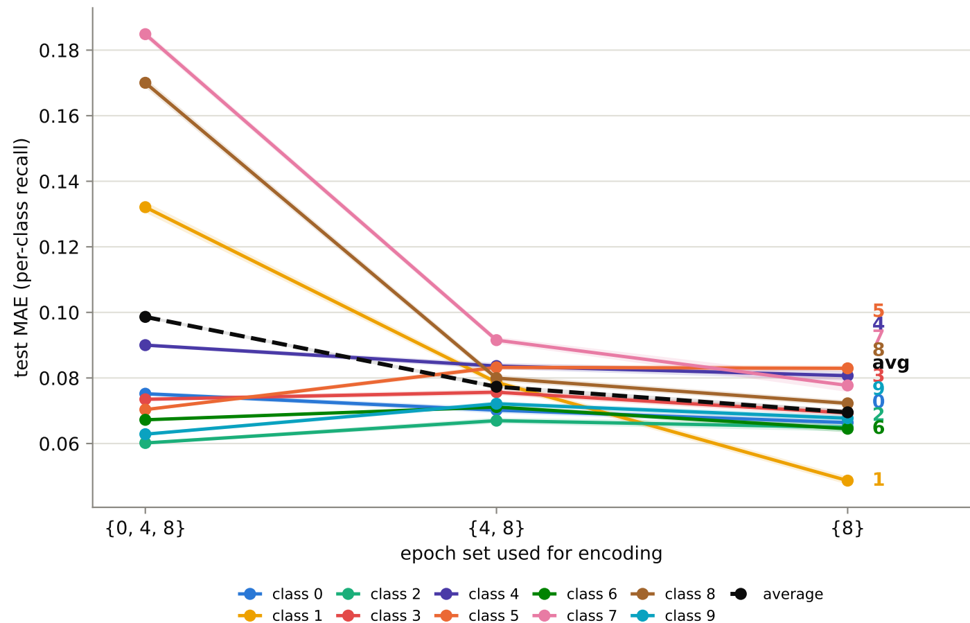
Per-class recall prediction error from SANE embeddings (7a92c ckpt50) — mean \pm std over 10 random 70/15/15 splits
