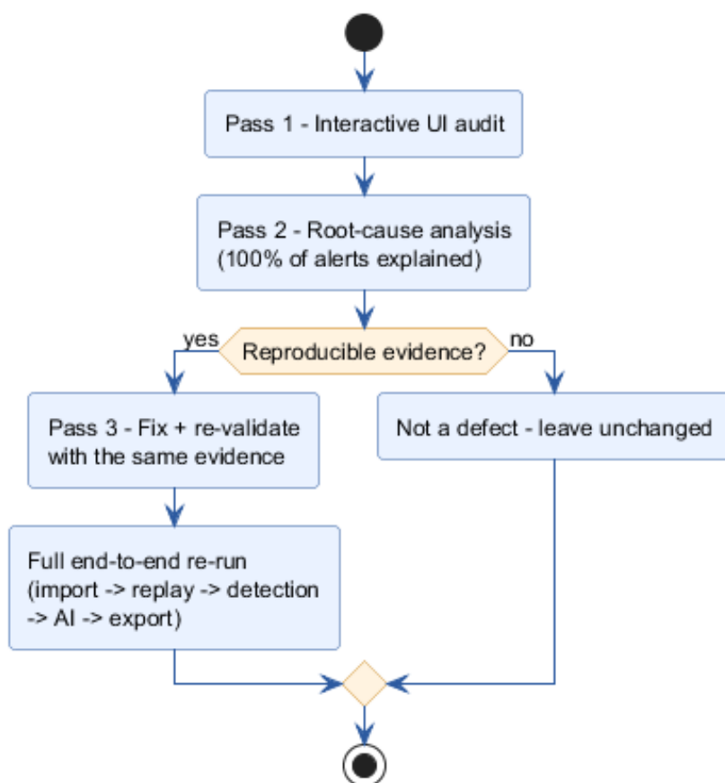
Figure 5.1: Validation workflow: three passes, gated by reproducible evidence.
