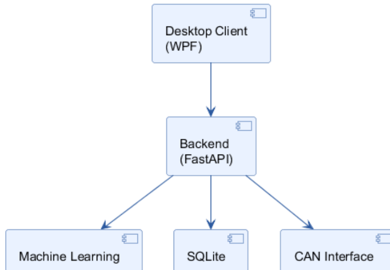
Figure 3.2: Overall layered architecture of CANvisionNative.
