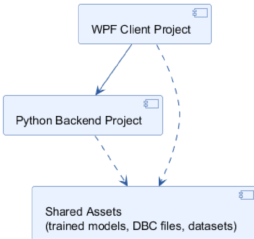
Figure 4.1: Repository organization: the WPF client, the Python backend, and shared assets.
