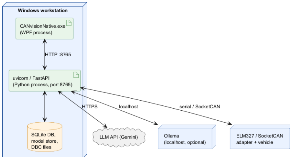
Figure 3.13: Deployment diagram: single-workstation deployment with external LLM and hardware links.
