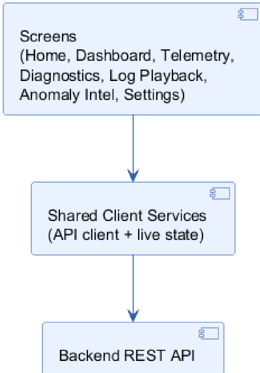
Figure 3.3: Frontend architecture: MVVM views bound to ViewModels, backed by two shared services.
