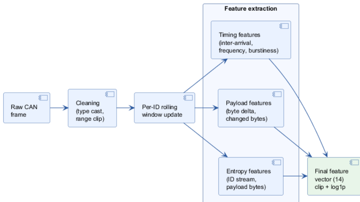
Figure 3.8: Feature engineering pipeline: from a raw frame to the final 14-feature vector.
