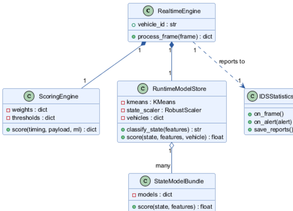
Figure 3.12: Simplified class diagram of the backend detection core.
