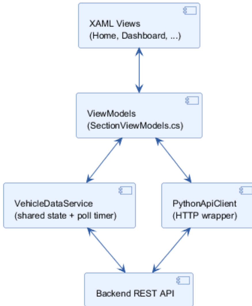
Figure 3.3: Frontend architecture: MVVM views bound to ViewModels, backed by two shared services.
