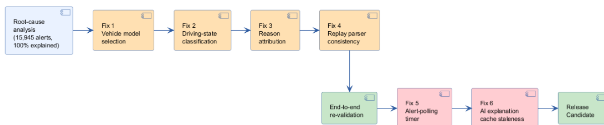
Figure 5.10: Bug-fix timeline: from root-cause analysis to the final Release Candidate.
