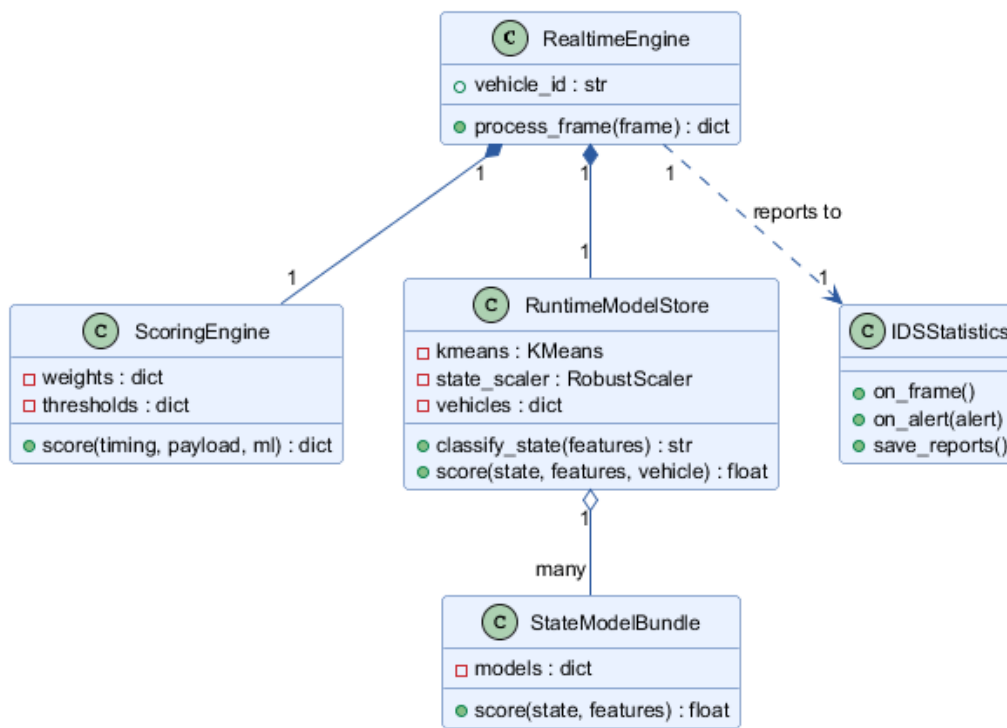
Figure 3.9: Simplified class diagram of the backend detection core.
