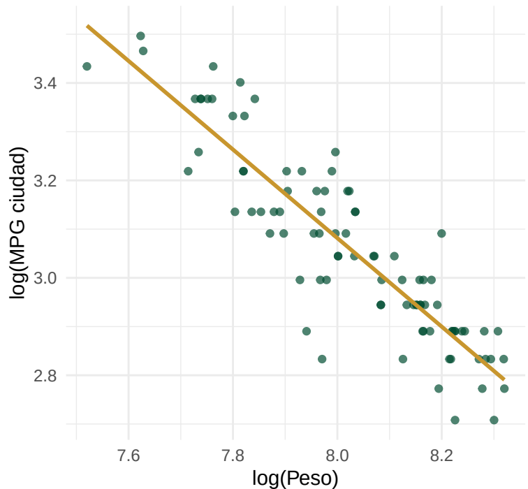
Transformado: \log(\text{Weight}) vs \log(\text{MPG.city})
