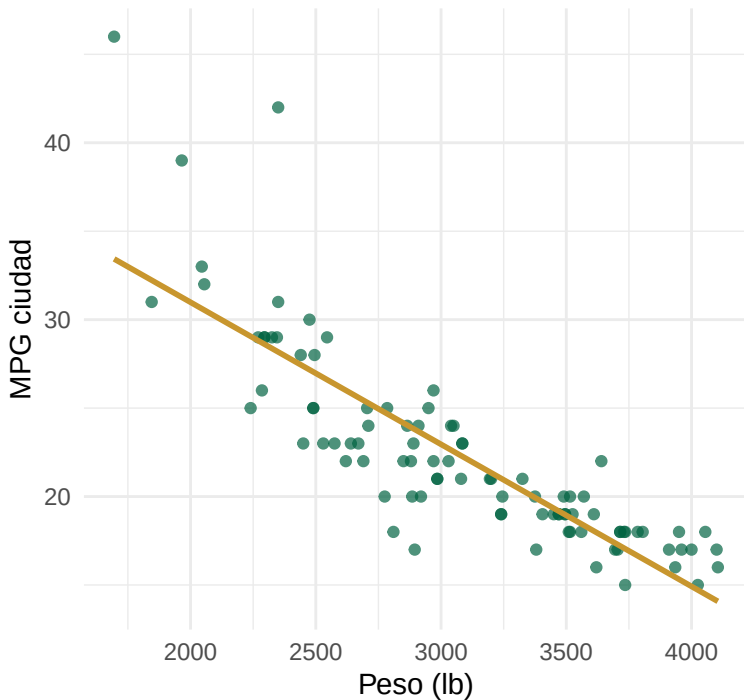
Original: Weight vs MPG.city
