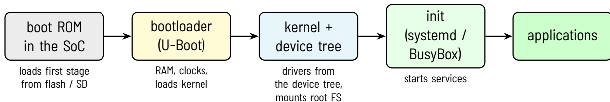
Figure 8.4.1: Boot chain of an embedded Linux system
