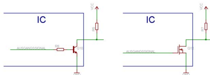
Figure 6.2.3: Open-drain output with external pull-up resistor
