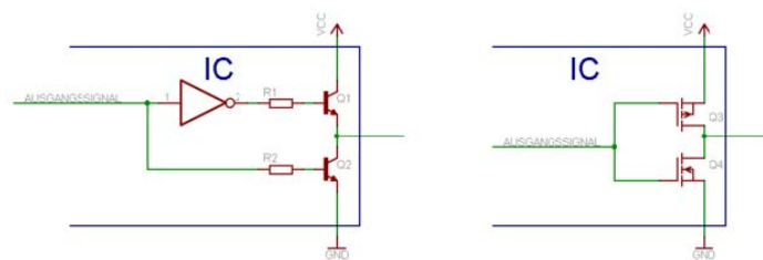
Figure 6.2.2: Push-pull output
