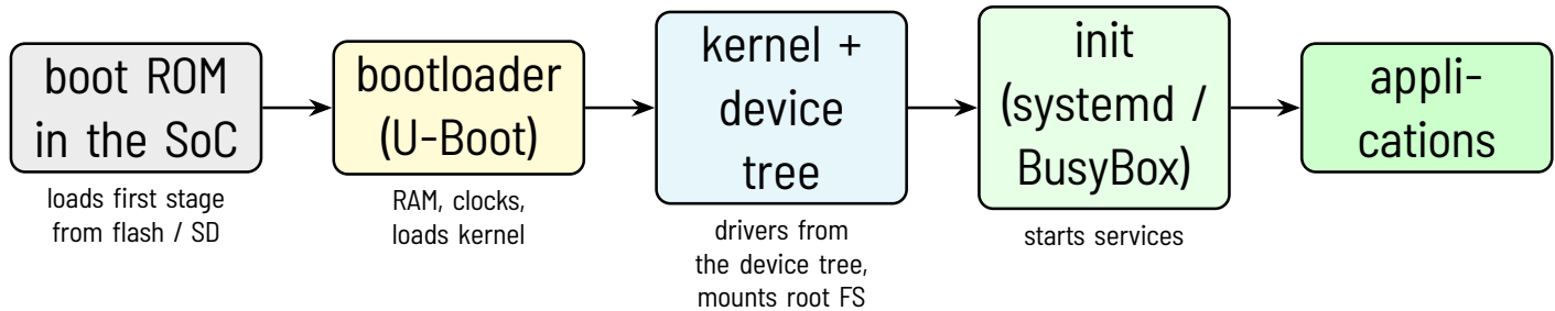
Figure 8.4.1: Boot chain of an embedded Linux system
