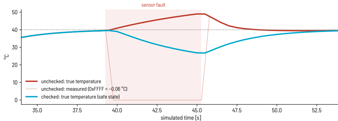
Figure 8.4.4: The program reads 0xFFFF = -0.06\text{ }^{\circ}\text{C} , drives the heater at 100 % and overheats the chamber – while its own log shows a cold chamber
