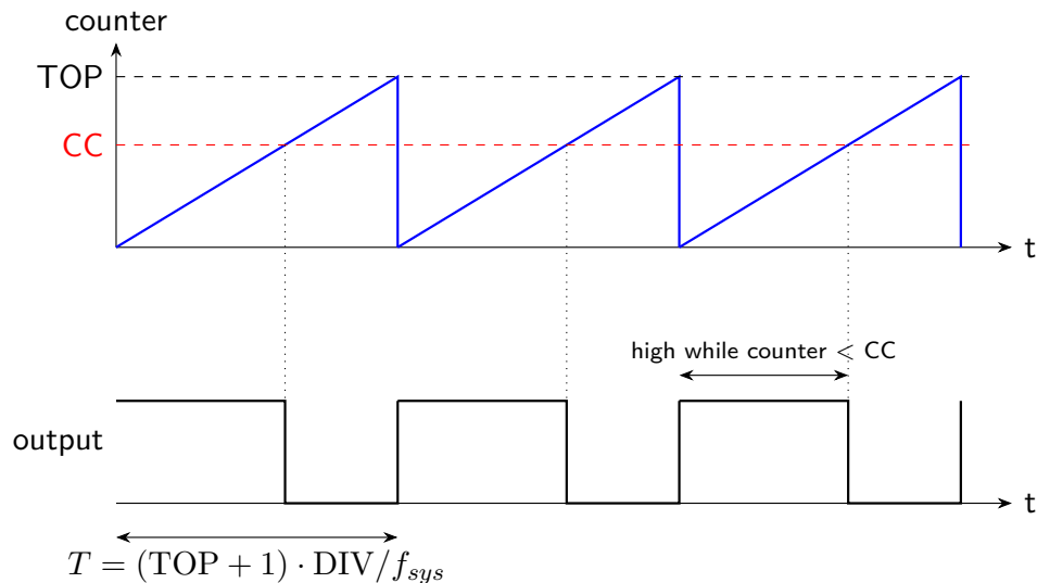
Figure 6.4.1: PWM: the output is high while the counter is below the compare value
