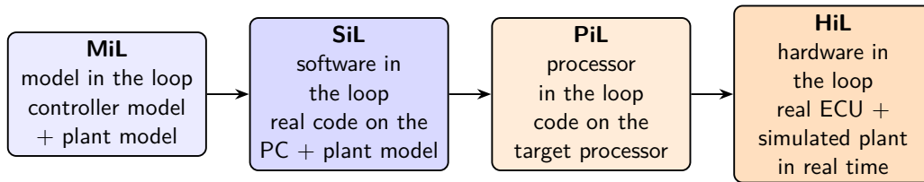
Figure 3.1.2: Test levels from the model to the real hardware
