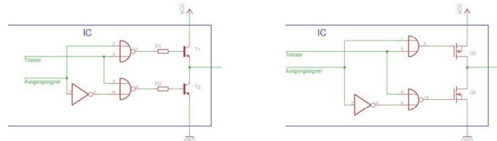
Figure 6.2.4: Tri-state output
