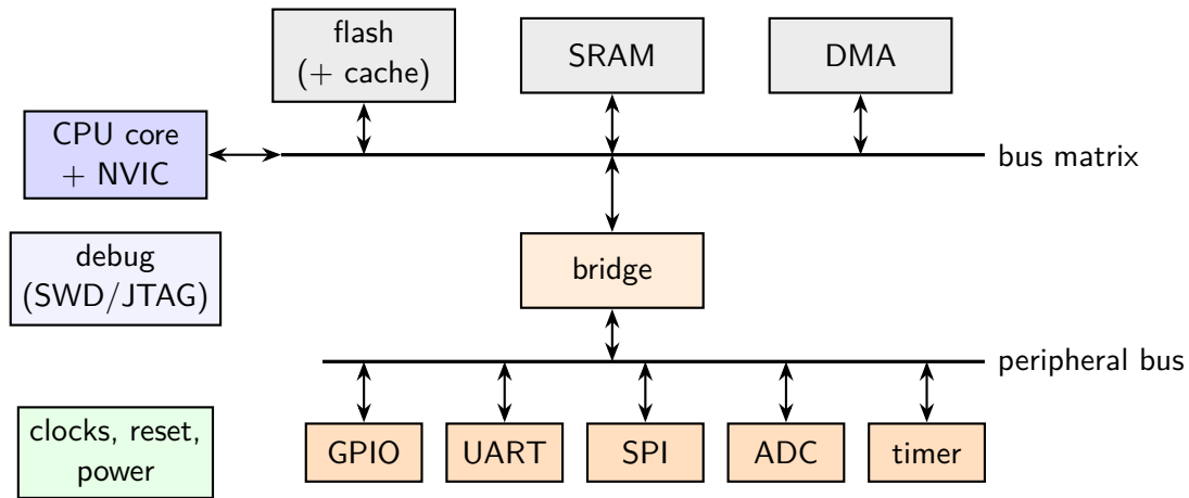
Figure 4.3.1: Typical structure of a 32 bit microcontroller
