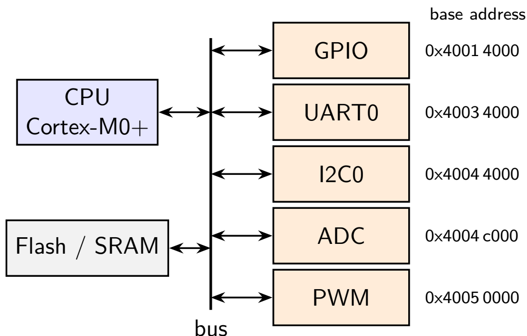
Figure 6.1.1: Peripherals are register blocks in the memory map (RP2040 addresses)
