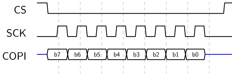
Figure 6.6.5: SPI mode 0: data changes on the falling edge and is sampled on the rising edge (dashed), MSB first
