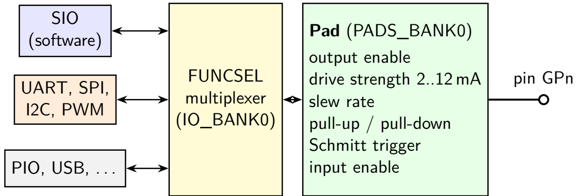
Figure 6.2.1: Path from the peripherals to a GPIO pin of the RP2040
