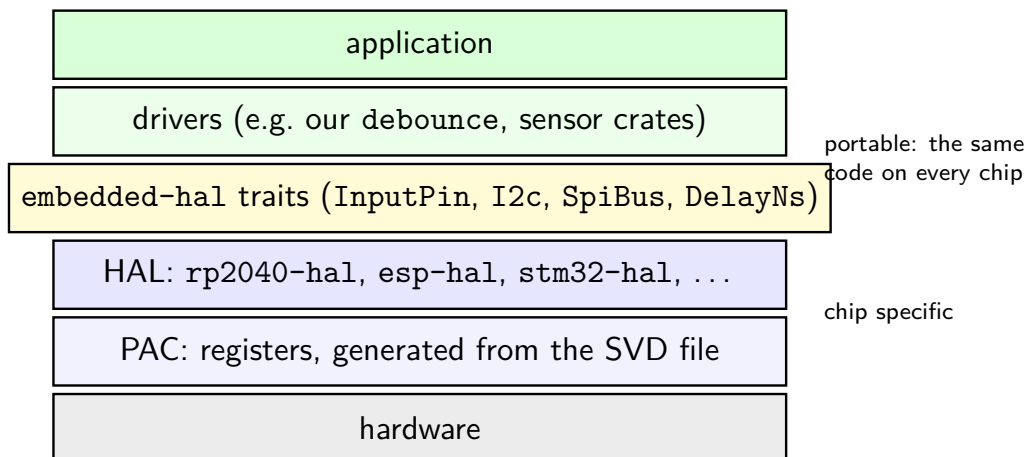
Figure 5.4.1: Layers of the embedded Rust ecosystem
