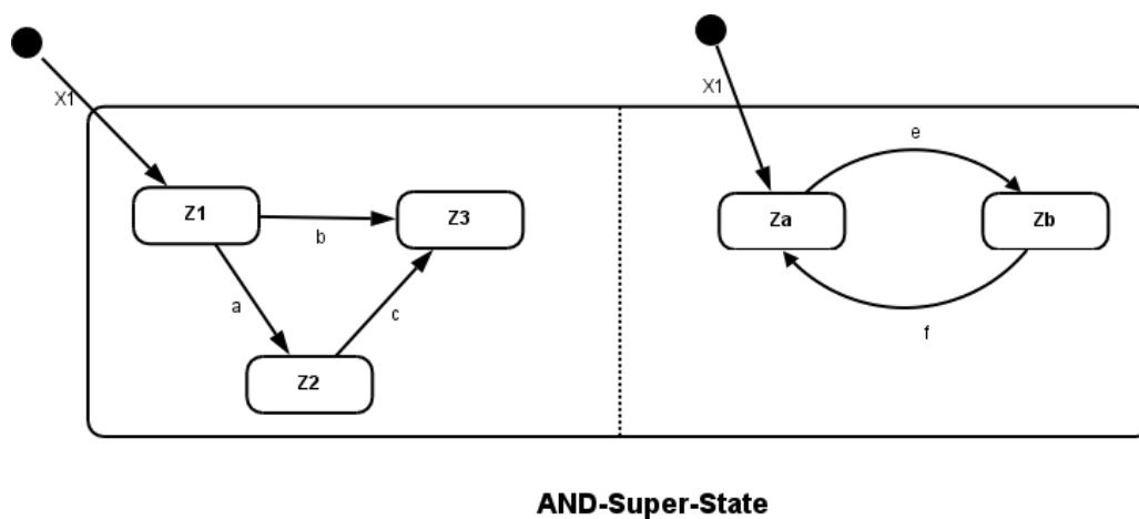
Figure 2.2.6: Example of an AND-super-state
