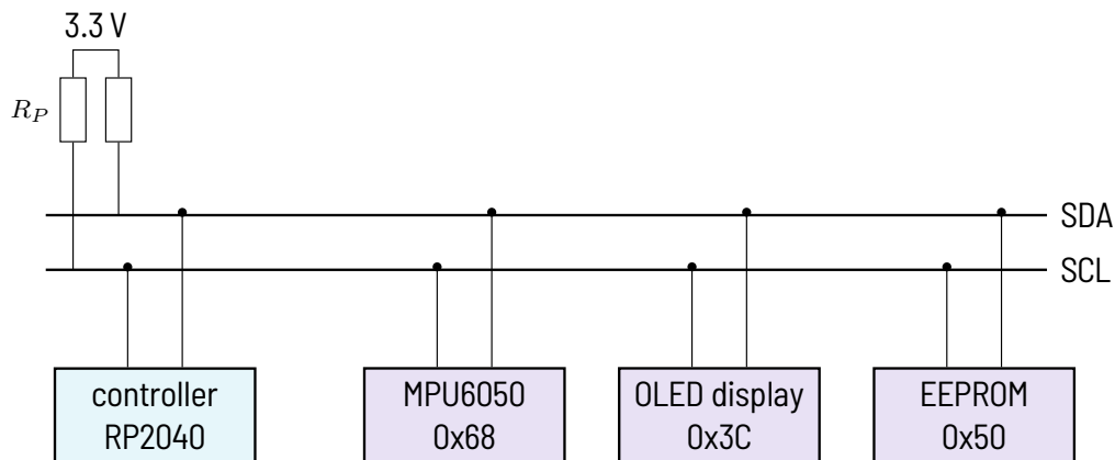
Figure 6.6.2: I 2 C bus: all devices share SDA and SCL, pull-up resistors R_P define the high level
