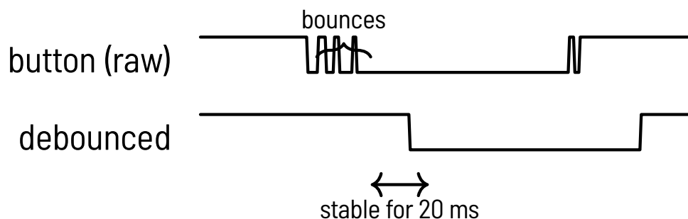
Figure 6.2.5: Bouncing button and debounced signal
