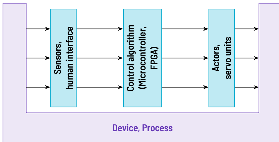
Figure 1.1.1: Block diagram of an embedded system
