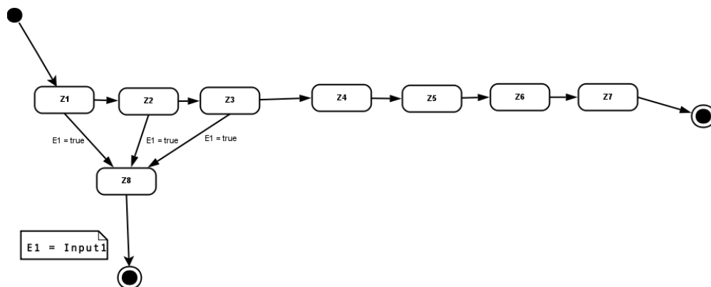
Figure 2.2.2: FSM in more detail
