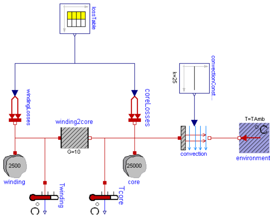
Figure 3.2.1: OpenModelica model of a heat transfer
