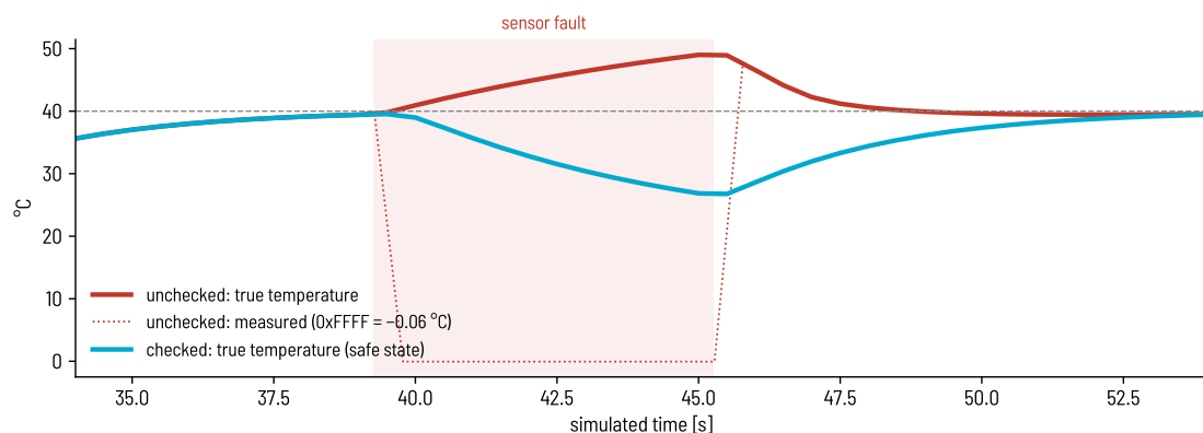
Figure 8.4.4: The program reads 0xFFFF = -0.06^{\circ}\text{C} , drives the heater at 100 % and overheats the chamber – while its own log shows a cold chamber
