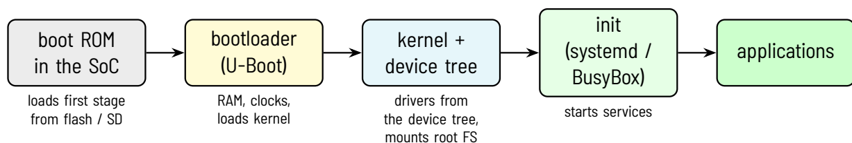
Figure 8.5.1: Boot chain of an embedded Linux system
