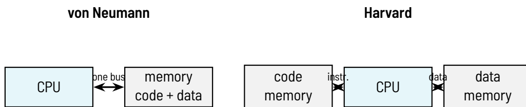
Figure 4.1.1: One bus for code and data, or separate buses
