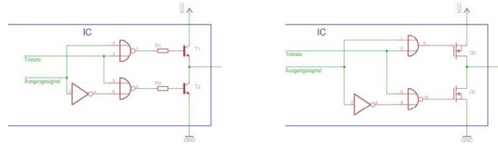
Figure 6.2.4: Tri-state output
