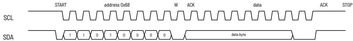
Figure 6.6.3: I 2 C write: START, address 0x68 with R/\overline{W} = 0 , ACK, data byte, ACK, STOP
