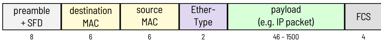
Figure 7.2.1: Ethernet frame (field sizes in bytes)
