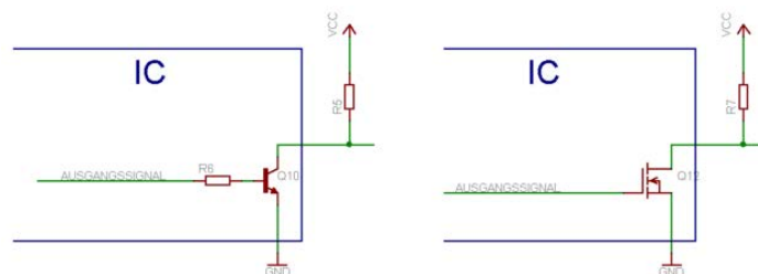
Figure 6.2.3: Open-drain output with external pull-up resistor
