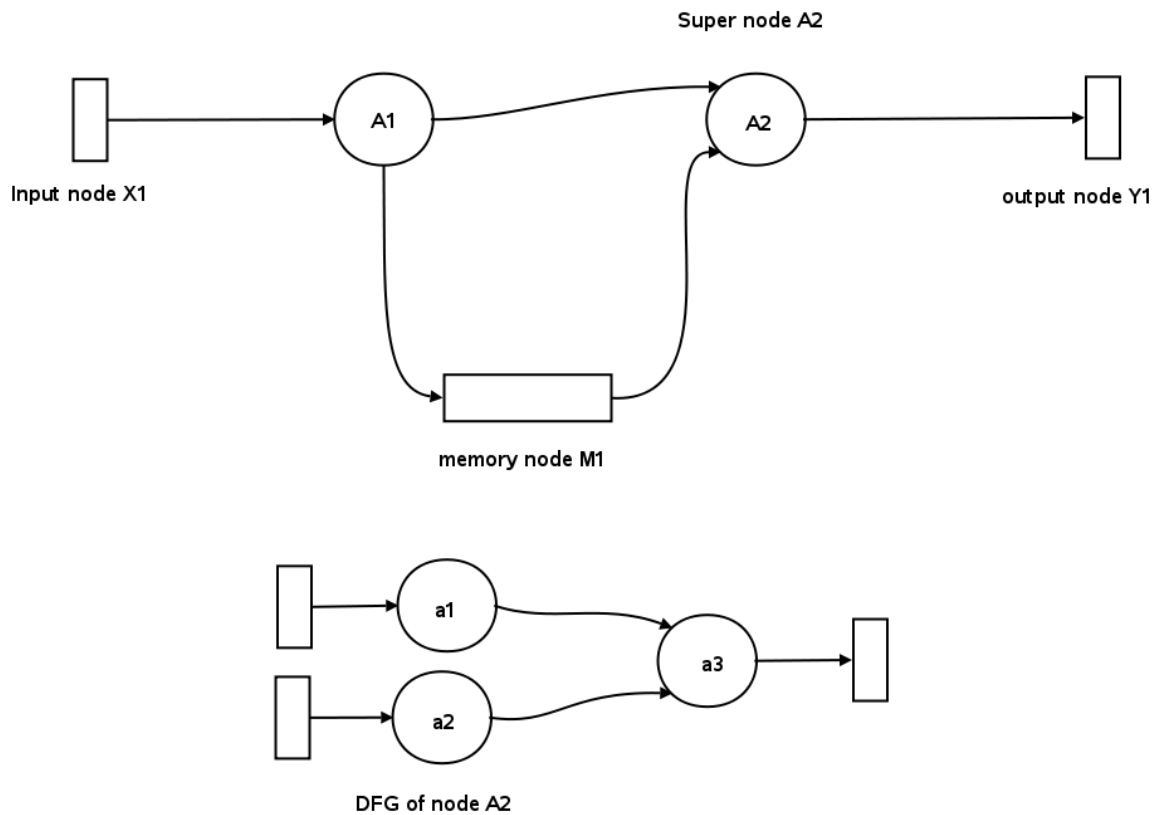
Figure 2.4.1: Data flow graph
