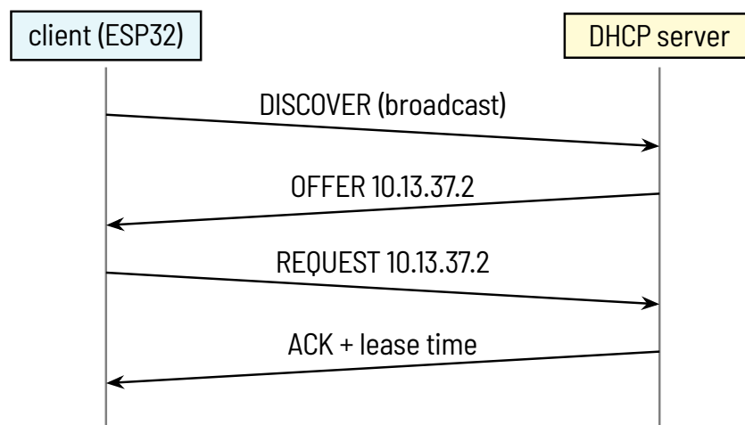
Figure 7.3.2: DHCP: Discover, Offer, Request, Acknowledge
