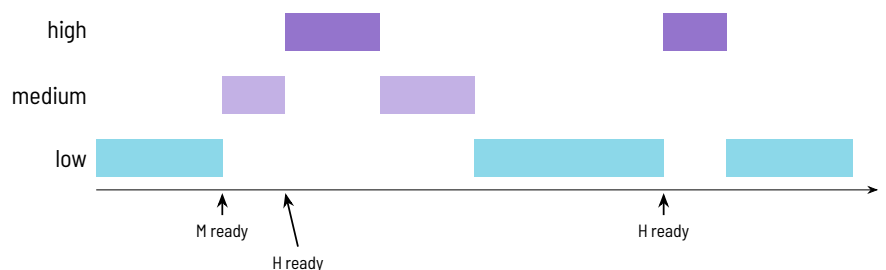
Figure 8.2.2: H preempts M, M preempts L; a task continues where it was interrupted
