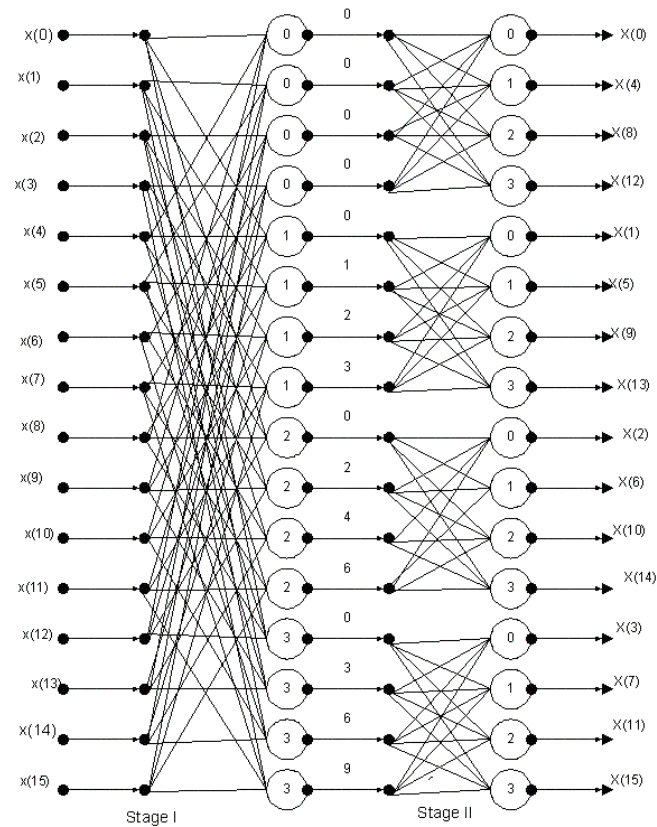
Figure 2.4.2: DFG of an FFT algorithm
