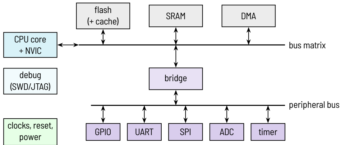
Figure 4.3.1: Typical structure of a 32 bit microcontroller
