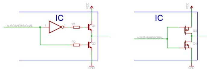
Figure 6.2.2: Push-pull output
