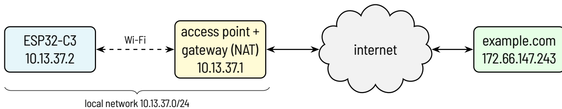
Figure 7.3.1: Our simulated device: everything outside 10.13.37.0/24 goes to the gateway
