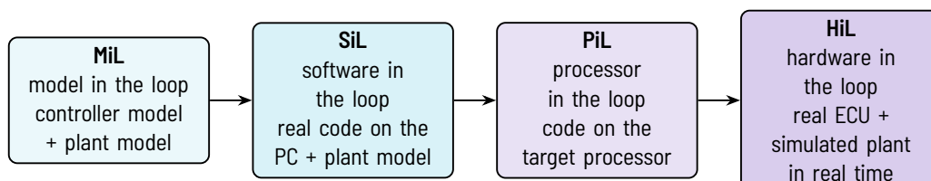
Figure 3.1.2: Test levels from the model to the real hardware
