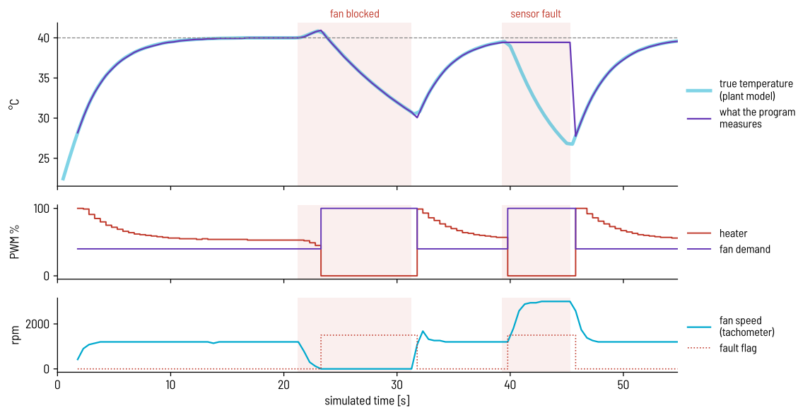
Figure 8.4.3: Blocked fan: alarm after 2.0 s (rotor slows down, then two slow 500 ms windows), heater off. Silent sensor: alarm after 0.5 s (queue timeout), heater off – the program shows the last value, the chamber cools down. Both faults clear by themselves.
