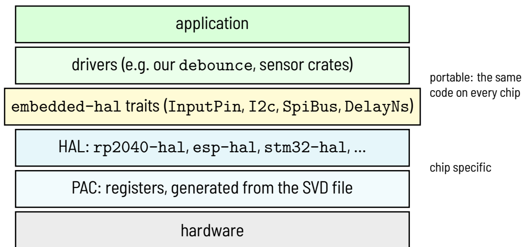
Figure 5.4.1: Layers of the embedded Rust ecosystem
