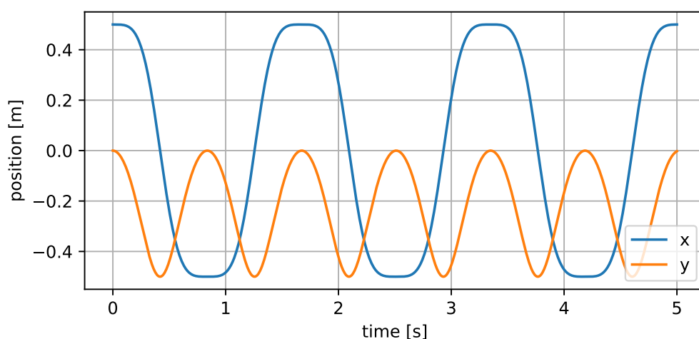
Figure 3.2.4: Horizontal and vertical position of the pendulum, started with the rod horizontal
