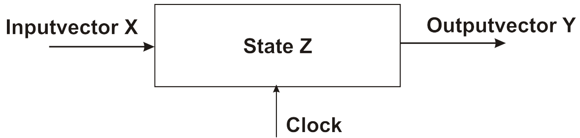
Figure 2.2.1: Block diagram of an FSM
