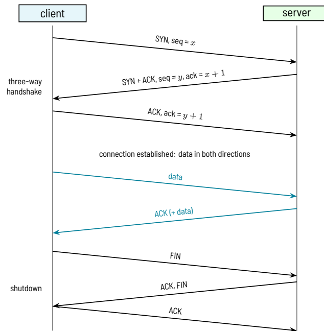
Figure 7.4.1: TCP: three-way handshake, data transfer and shutdown
