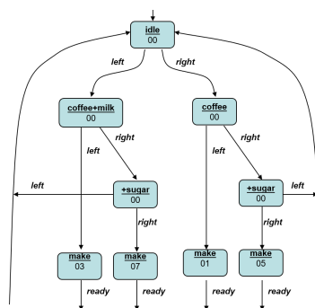
Figure 2.3.1: Coffee machine FSM
