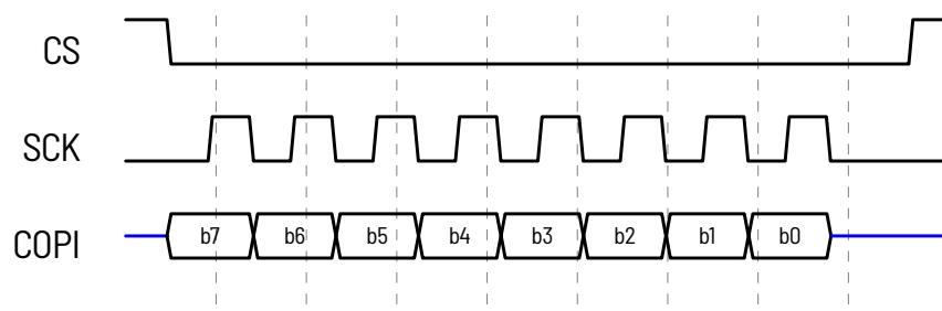
Figure 6.6.5: SPI mode 0: data changes on the falling edge and is sampled on the rising edge (dashed), MSB first
