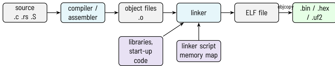
Figure 5.1.1: From source code to the image in the flash
