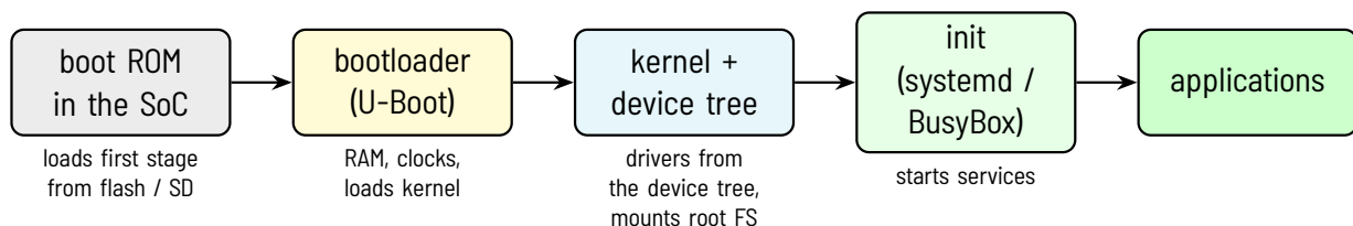
Figure 8.5.1: Boot chain of an embedded Linux system
