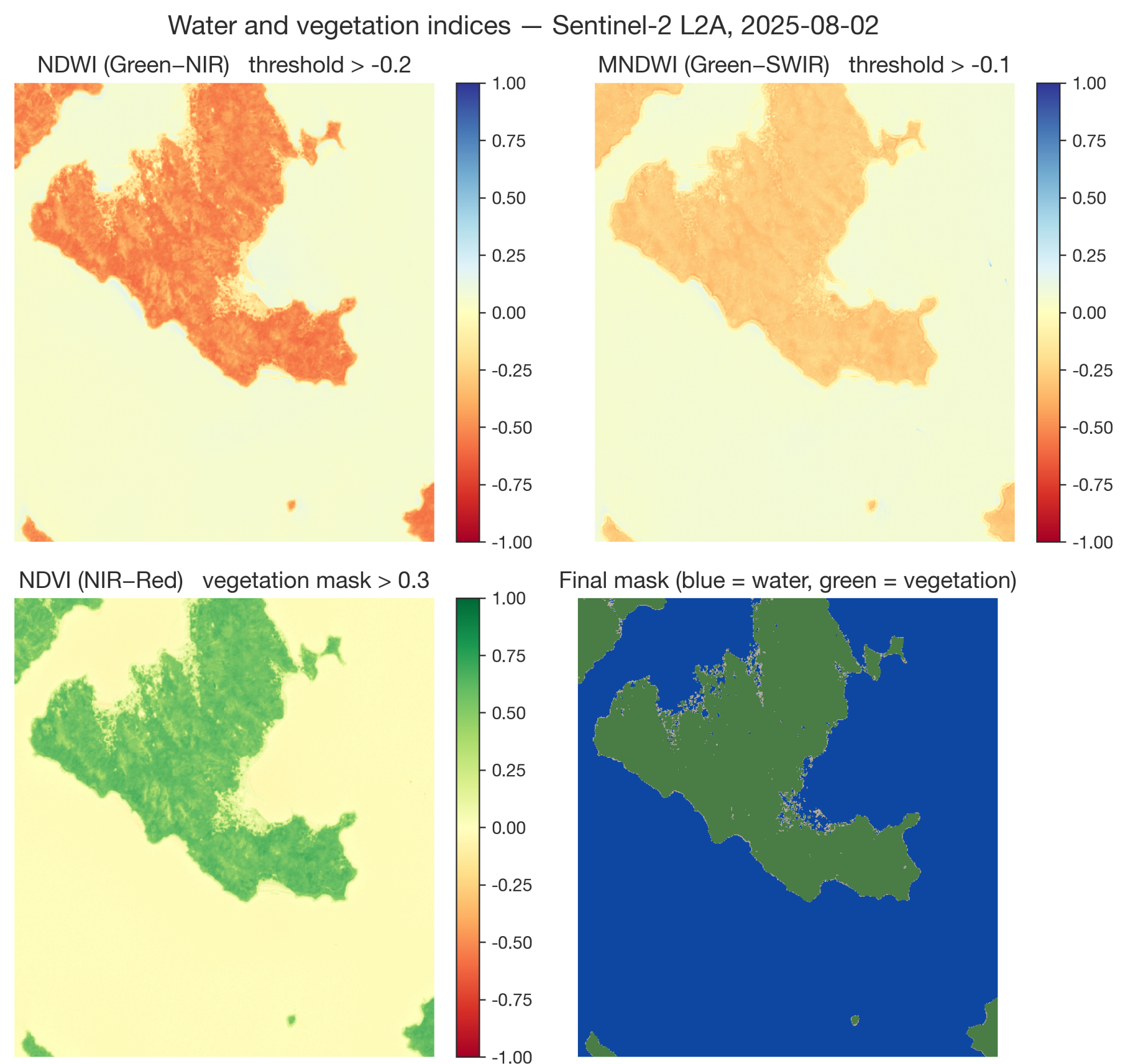
NDWI, MNDWI, NDVI and the final water/vegetation mask, Sentinel-2 L2A, 2025-08-02. Contains modified Copernicus Sentinel data [2025].
