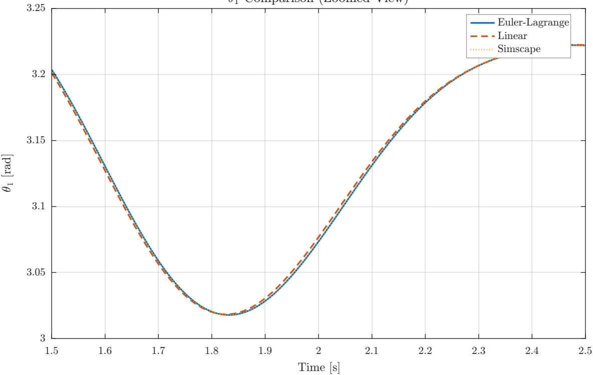
\theta_1 Comparison (Zoomed View)
