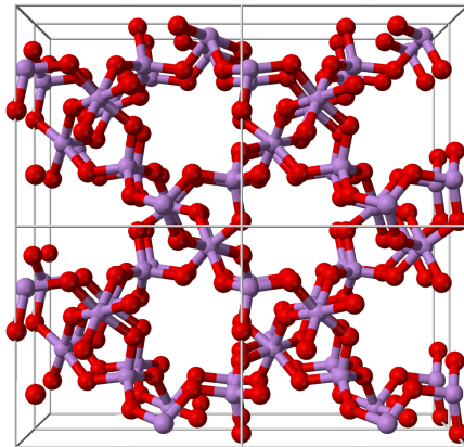
Krystalová struktura As 4 O 10 . 94
