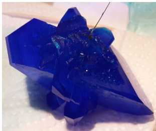
Krystaly modré skalice. 92
