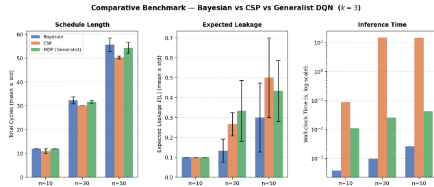
Figure 2: Comparative benchmark across all three solvers for k = 3 , averaged over seeds {42, 43, 44}. Error bars show \pm 1 standard deviation. Wall-clock time is shown on a log scale; MDP reflects inference only (training excluded).
