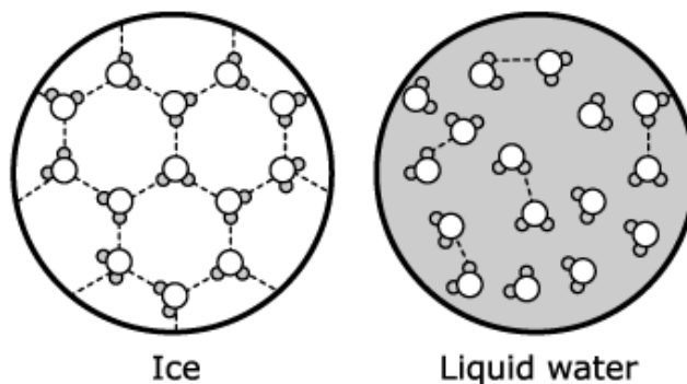
Figure 1. Water Particles in Ice and in Liquid Water
