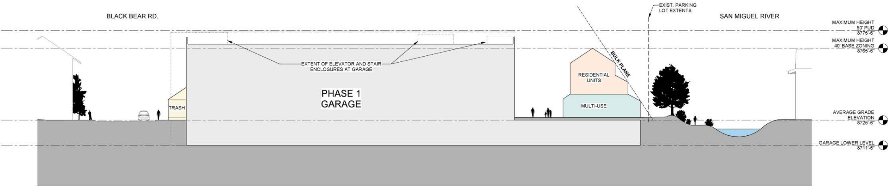
1 SITE SECTION - NORTH / SOUTH A301
