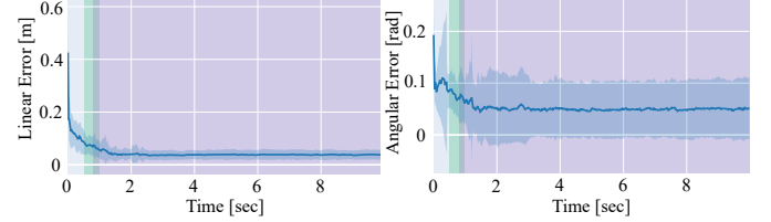
Fig. 4: State estimation error of our method. Shows mean \pm 1 standard deviation across 50 episodes. The green region shows the area where vision is available, and the purple region shows the area where there is contact between the robot and box.
