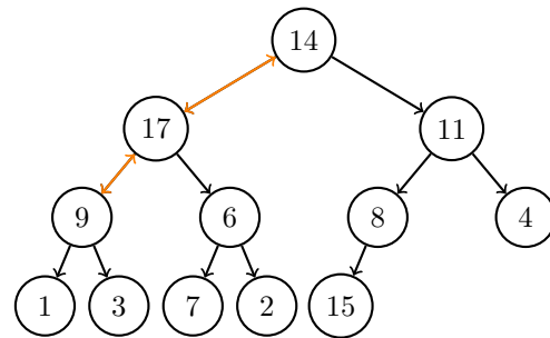
Heapify root
