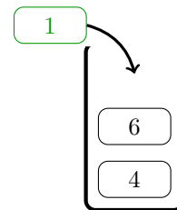
Push
