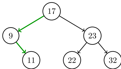
Search for 11
