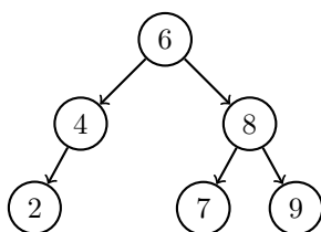
Leaf Deletion
