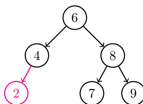
Delete 2
